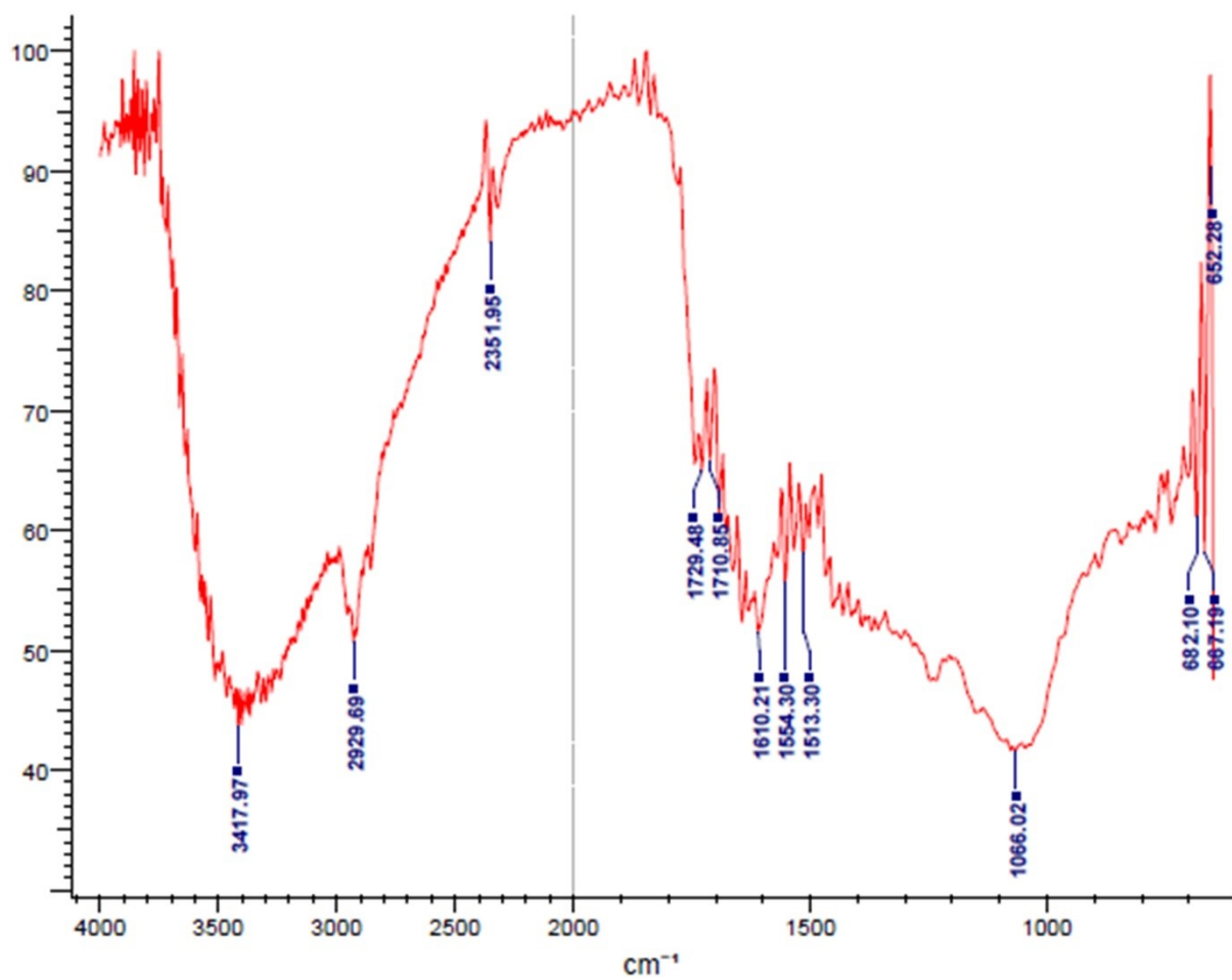
Figure 1S. FT-IR spectrum of aqueous seed extract of Pimpinella anisum .
