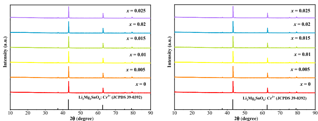
Fig. S1. XRD patterns of LMTAO: x\text{Cr}^{3+} and LMTGO: x\text{Cr}^{3+}
