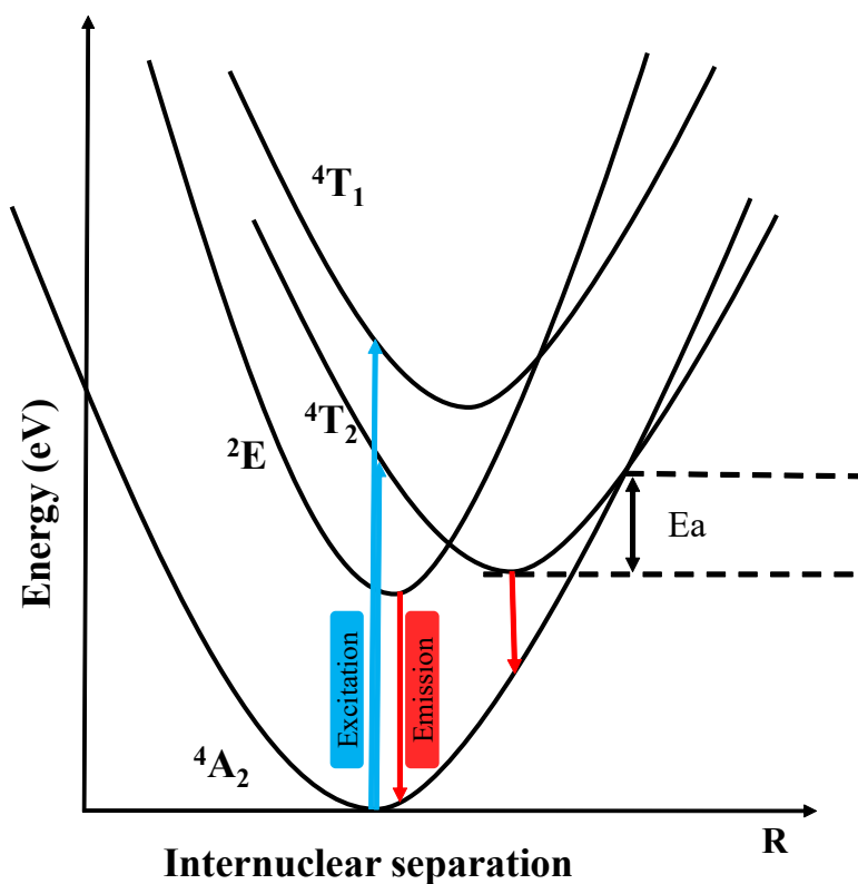
Fig. S2. The configurational coordinate diagram for \text{Cr}^{3+} ions in \text{Li}_2\text{Mg}_3\text{TiO}_6 \cdot \text{Cr}^{3+} phosphors.
