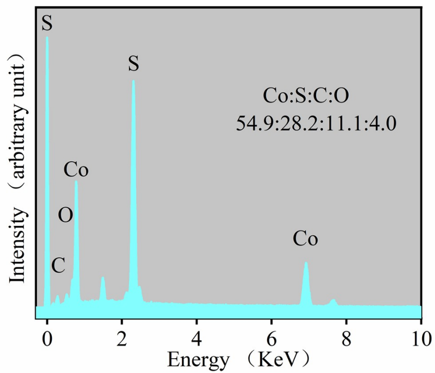
Figure S1 EDS spectra of \text{Co}_{1-x}\text{S}
