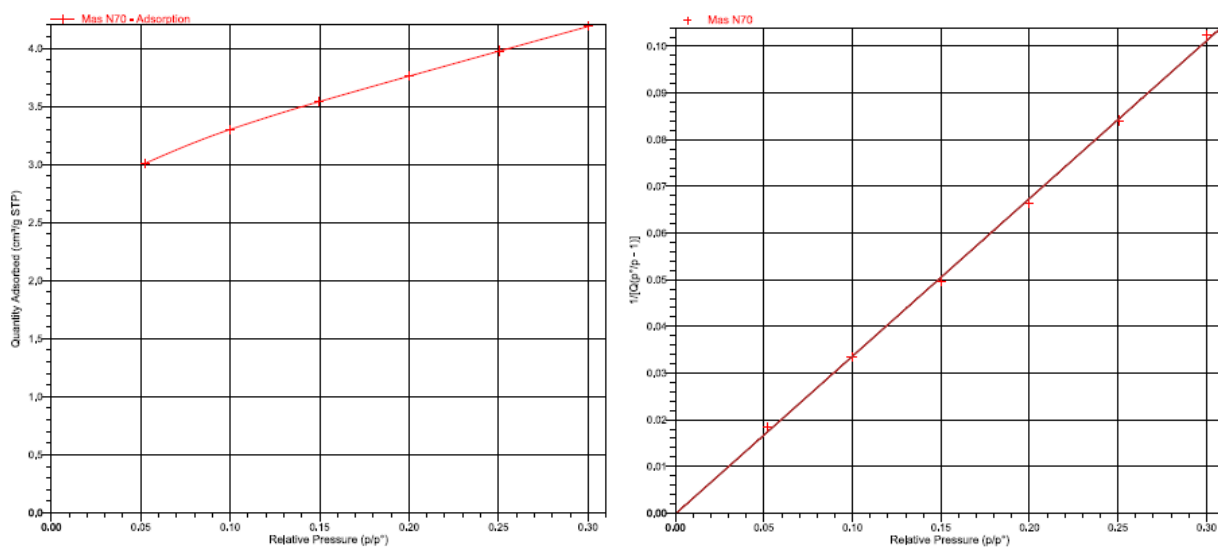
Fig. S2 (a) N 2 adsorption–desorption isotherm and (b) BET surface area plot of MAS-N70.
