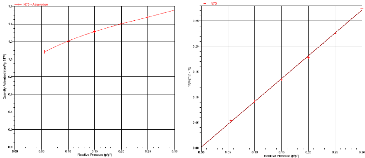
Fig. S1 (a) N 2 adsorption–desorption isotherm and (b) BET surface area plot of N70.
