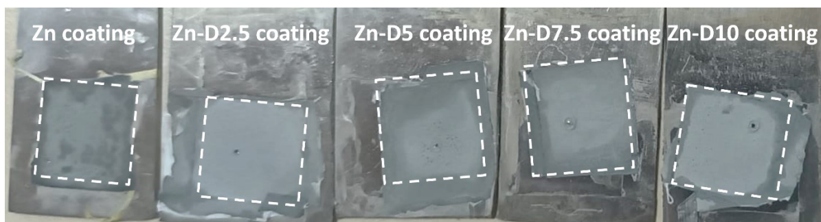
Figure SI 1: Digital camera images of as-prepared Zn-diamond composite coatings.
