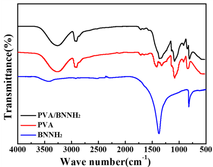
Fig.S1 FTIR spectra of BNNH 2 (blue), PVA (red) and PVA/BNNH 2 film (black).
