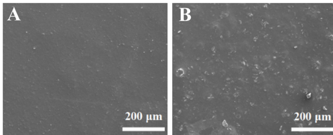
Fig.S2 The surface SEM images of PVA and PVA/BNNH 2 film with 30 wt % fillers.
