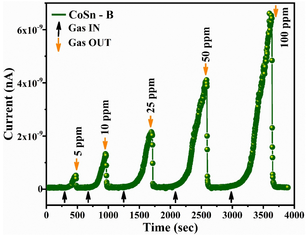
Fig. 1, Dynamic response curve for CoSn - B
