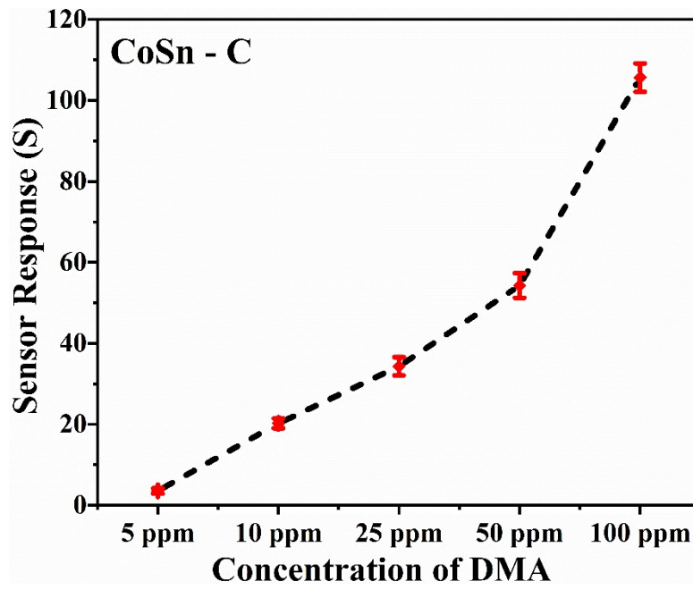
Fig. 4(b), gas response of CoSn - C film at different concentration of DMA
