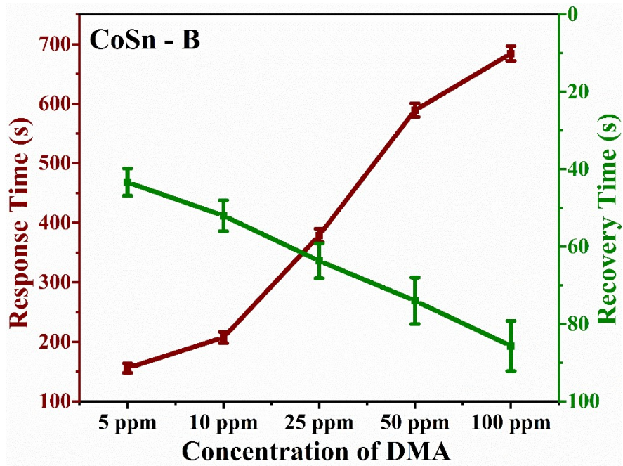
Fig. 3(a), CoSn - B at different concentration of DMA vs response time and recovery time.
