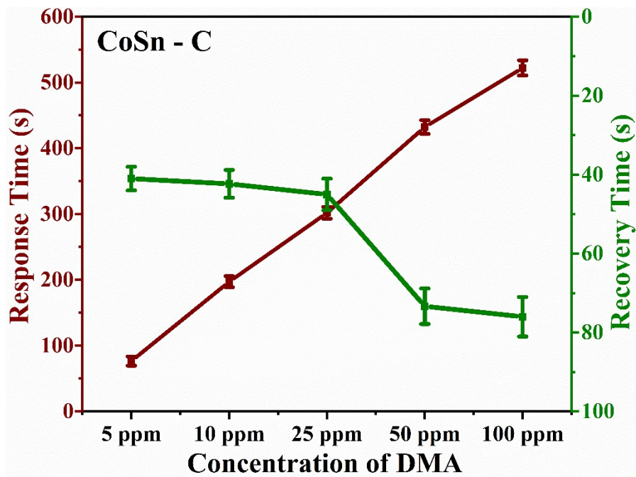
Fig. 4(a), CoSn - C at different concentration of DMA vs response time and recovery time.
