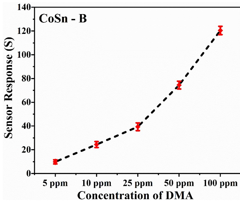
Fig. 3(b), gas response of CoSn - B film at different concentration of DMA
