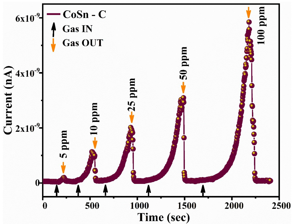
Fig. 2, Dynamic response curve for CoSn - C
