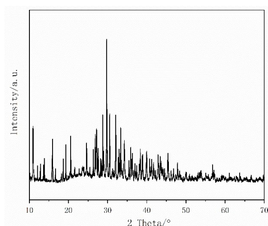
Fig. S2. XRD spectra of Ag-MOF@GO after three cycles.
