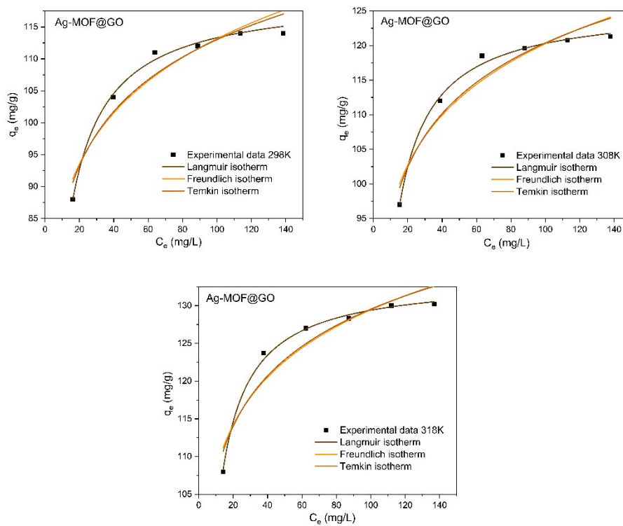
Fig. S1. Langmuir, Freundlich and Temkin isotherm models for the adsorption of MG dyes at three different temperatures using Ag-MOF@GO.
