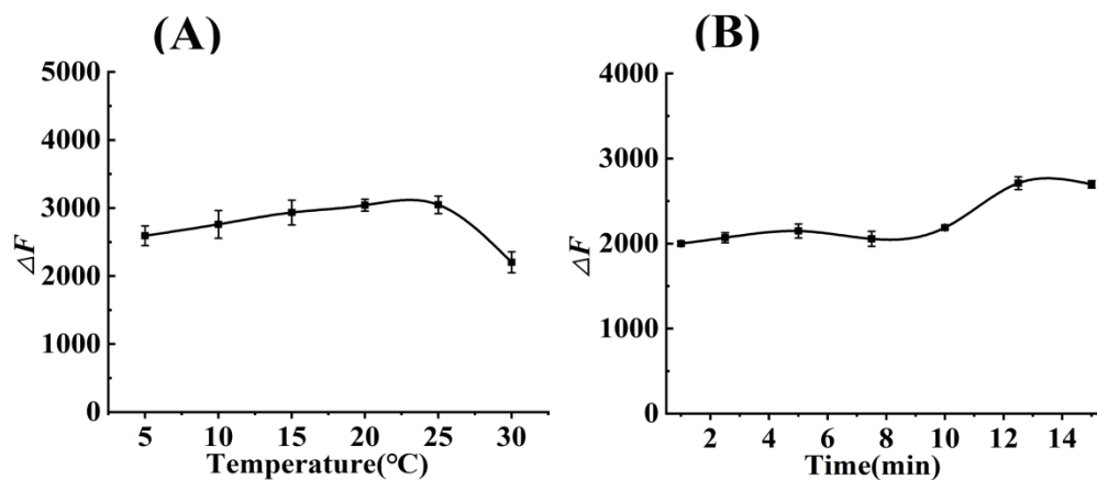
Figure S5. Optimization of FA detection conditions. (A) Reaction temperature. (B) Reaction time.
