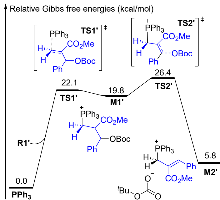
Fig. S1 Gibbs free energy profiles for the formation of complex intermediate M2'
