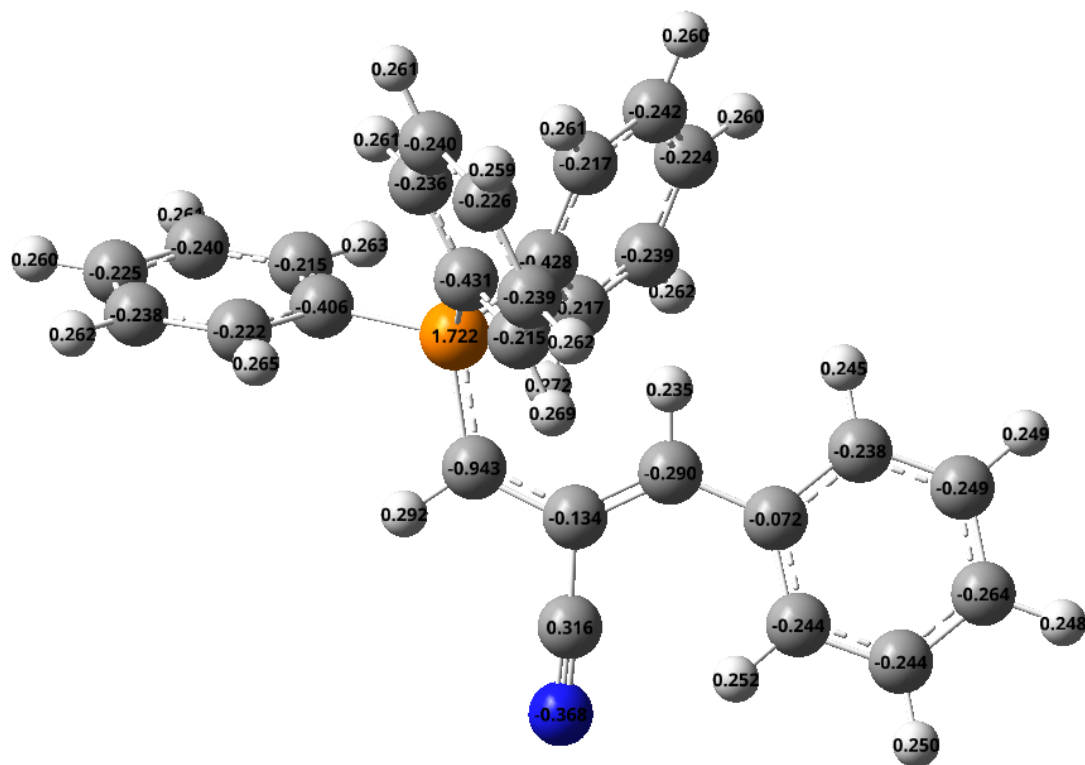
Fig. S3 NPA charge of \alpha - and \gamma -carbon atoms in the allylic phosphorus ylide
