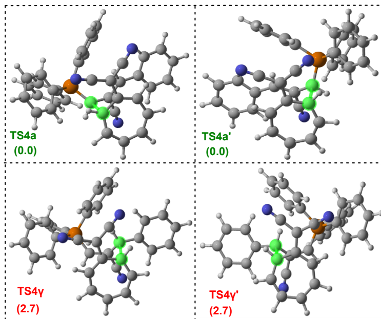
Fig. S2 3D structures and energies barriers involved in C-C bond formation process
