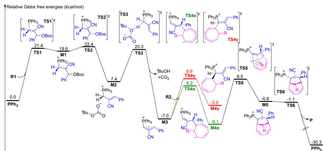
Fig. S4 The energy profile for the entire catalytic cycle
