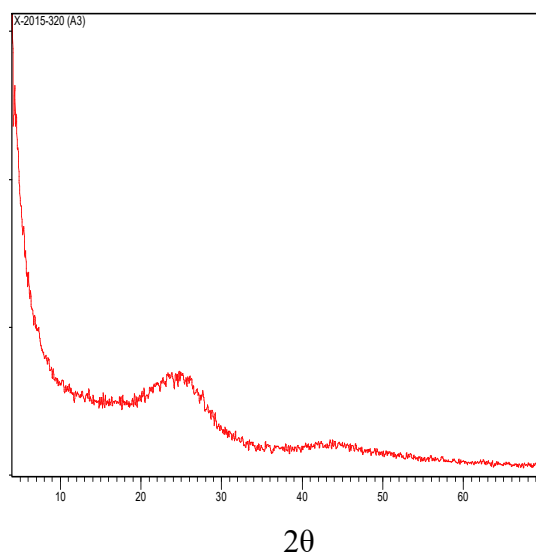
Figure S2. XRD pattern of activated carbon.
