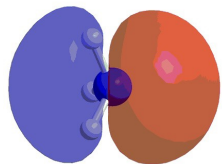
\text{NH}_3 , HOMO
