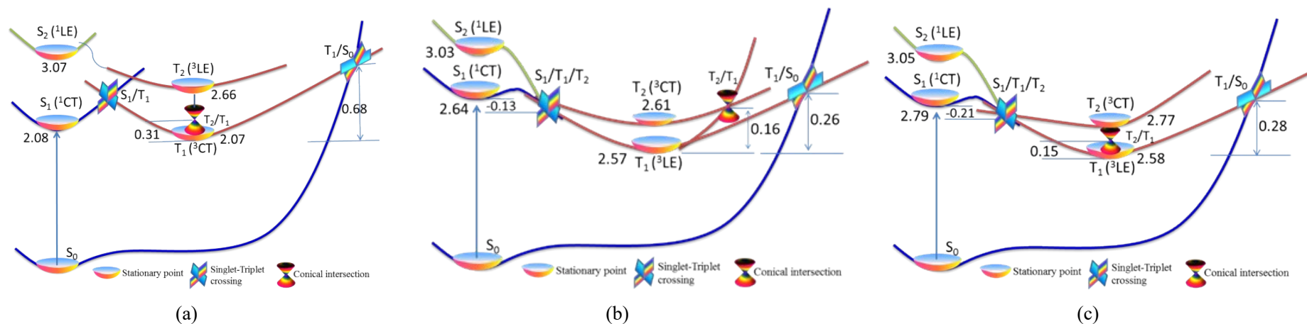
Fig. S4 Nonabatic potential energy surface diagrams of (a) AQ-PTZ, (b) AQ-PTZ-O and (c) AQ-PTZ-O 2 are from single-point calculation at the tuned- \omega *B97X-D3 level of theory in cyclohexane (with PCM mode). Minimum energy crossing point (MECP) of different spin states (S 1 /T 1 , T 1 /S 0 and S 1 /T 1 /T 2 ) and conical intersection of the same spin states (T 2 /T 1 ) were also obtained.
