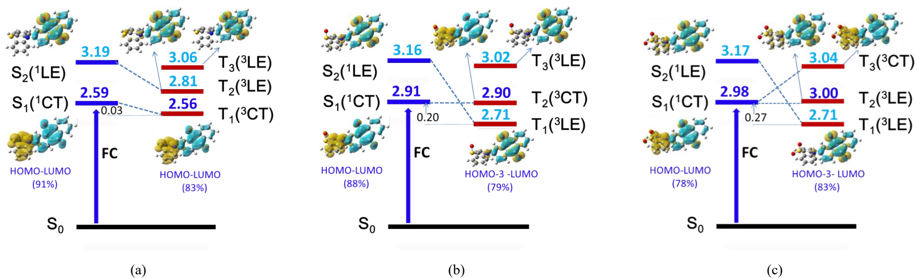
Fig. S3 Adiabatic energy transition diagrams of (a) AQ-PTZ, (b) AQ-PTZ-O and (c) AQ-PTZ-O 2 are from calculation by the tuned- \omega *B97X-D3 level of theory in cyclohexane (with PCM mode). The density difference distributions of the excited states are inserted into the diagrams. CT: charge transfer. LE: Local excitation. FC: Franck-Condon.
