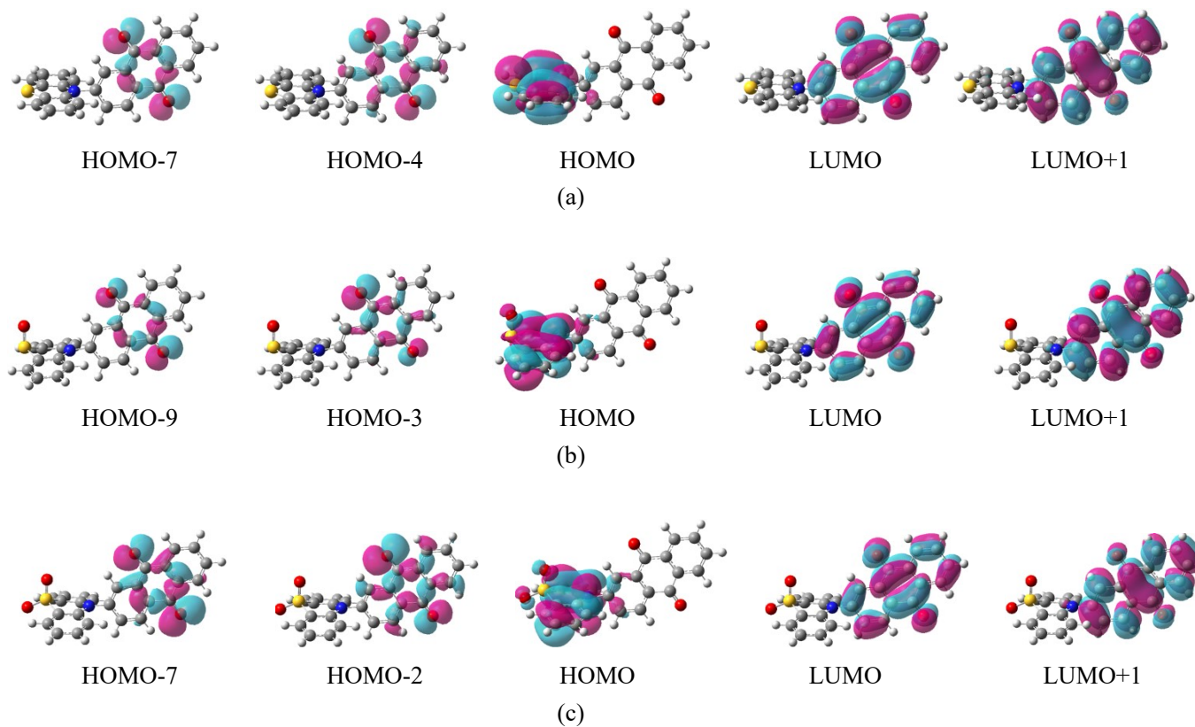
Fig. S2 Key transition active orbitals of (a) AQ-PTZ, (b) AQ-PTZ-O, and (c) AQ-PTZ-O 2 compounds from the tuned- \omega *B97X-D3 level of theory in cyclohexane (with PCM mode).
