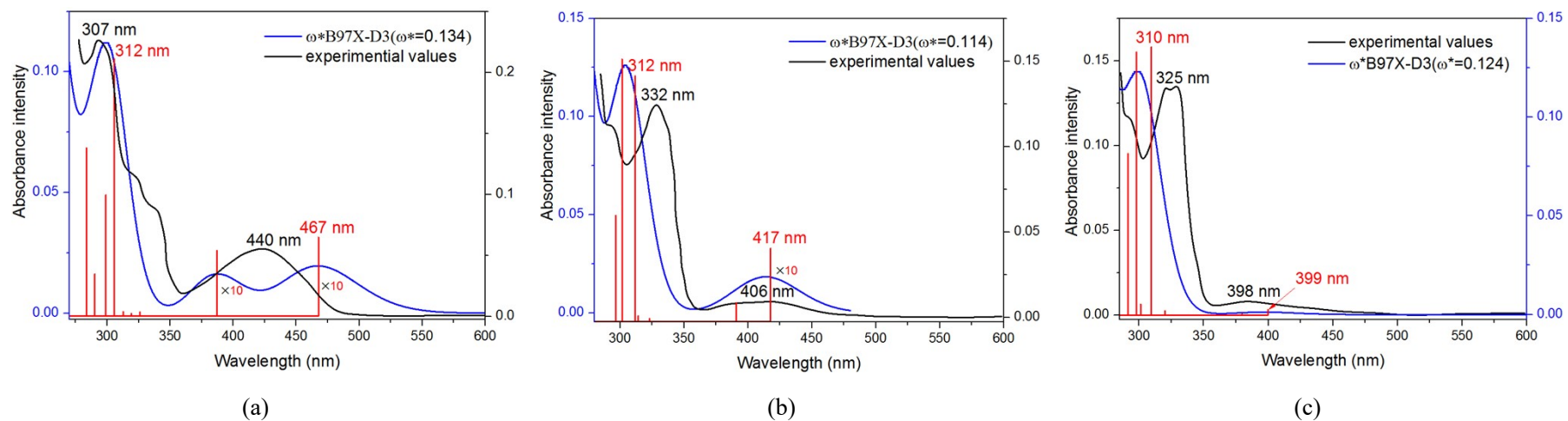
Fig. S1 Comparison of the calculated and the experimental absorption spectra of (a) AQ-PTZ, (b) AQ-PTZ-O and (c) AQ-PTZ-O 2 in cyclohexane (with PCM mode), and calculated at the TD-DFT at the tuned- \omega^* B97X-D3 level.
