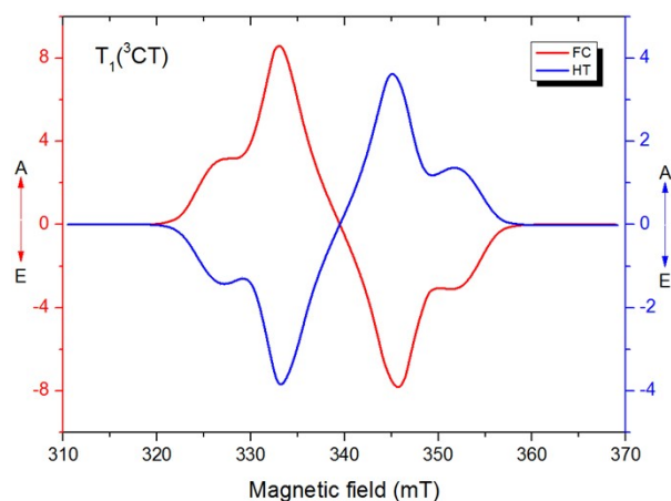
Fig. S6 Simulated EPR spectra of the charge-transfer triplet T_1(^3CT) of the AQ-PTZ-O compound.
