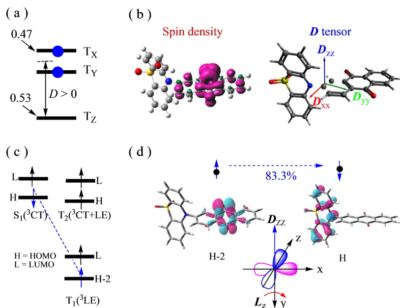
Fig. S7 (a) Relative populations in the zero-field T_1(^3LE) spin sublevels obtained for D > 0 of AQ-PTZ-O 2 ; (b) Spin density and the ZFS tensor ( D ) orientations of AQ-PTZ-O 2 ; (c) Schematic representation of the S_1 \leftrightarrow T_1 allowed ISC in AQ-PTZ-O 2 ; (d) Representative topologies of the spin-flip orbitals are depicted between the H-2 and L orbitals, demonstrating that SOC is effective as the angular momentum change ( L_z ) along the z-axis to cause the spin-flip.
