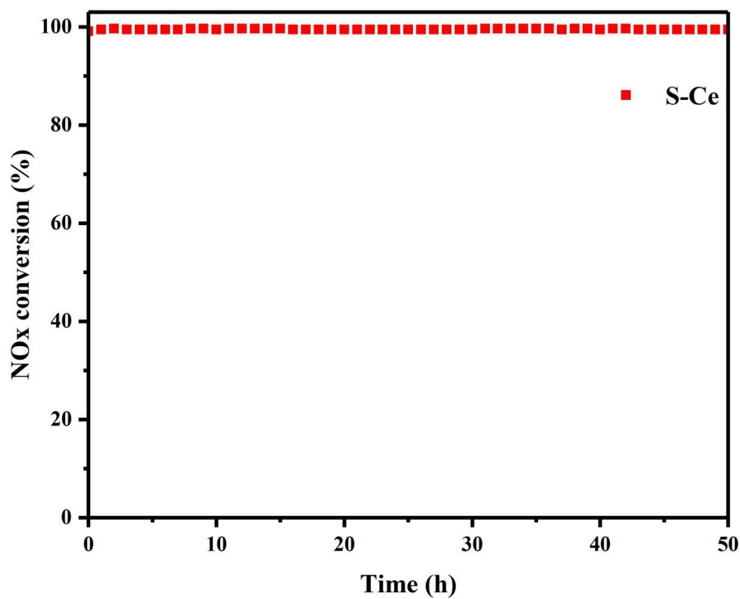
Fig. S1. the stability test of S-Ce catalysts
