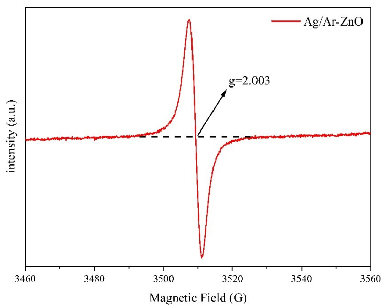
Fig. S1 EPR spectra of Ag/Ar-ZnO photocatalyst
