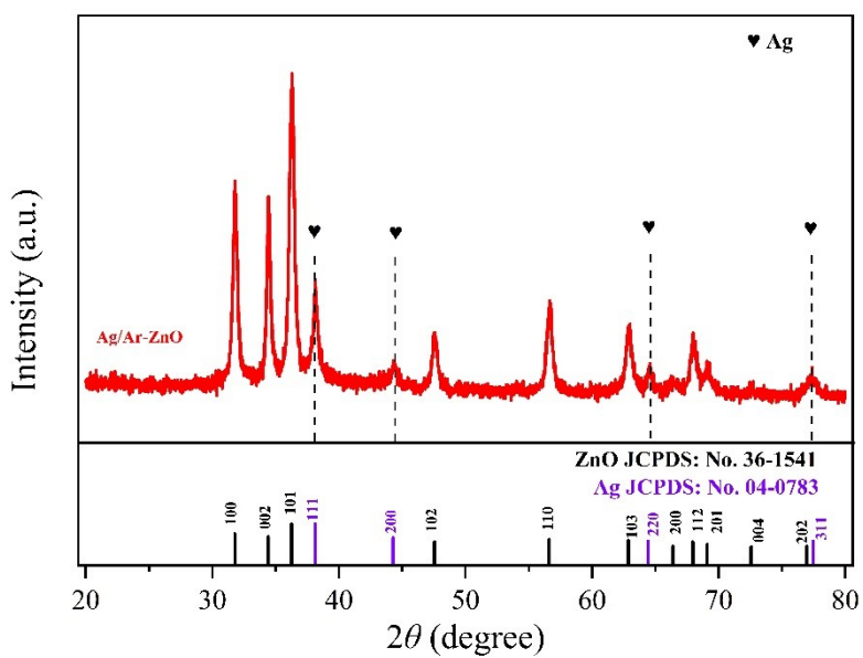
Fig. S2 XRD pattern of Ag/Ar-ZnO photocatalyst after the photocatalytic reaction
