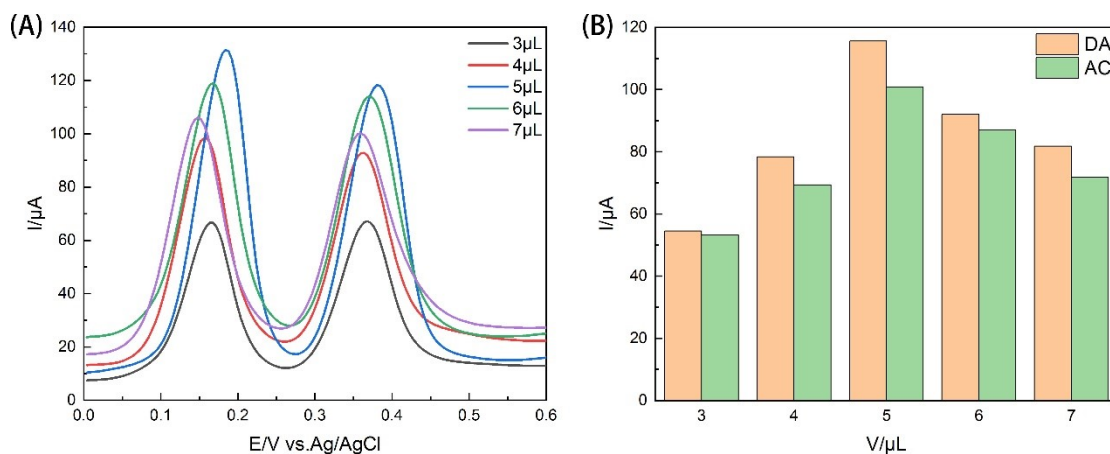
Fig.S1 (A) DPVs of C-ZIF-67/SP/GCE at different dropping amount, (B) Histogram of the relationship between dropping amount and peak height.
