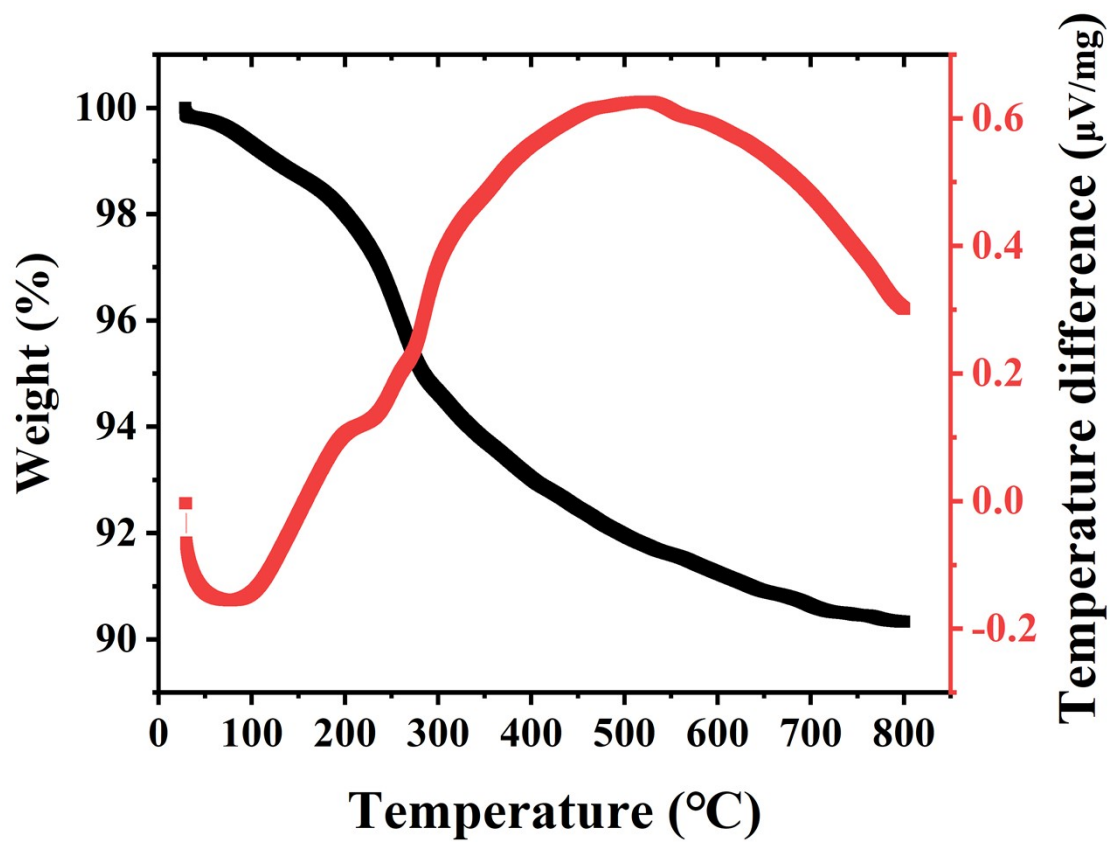
Fig. S2 The thermogravimetric differential curves of Fe 3 O 4 -HA@[TEAC][G].
