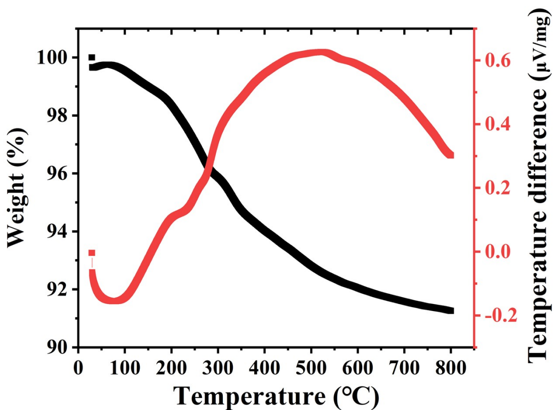
Fig. S1 The thermogravimetric differential curves of Fe 3 O 4 -HA.
