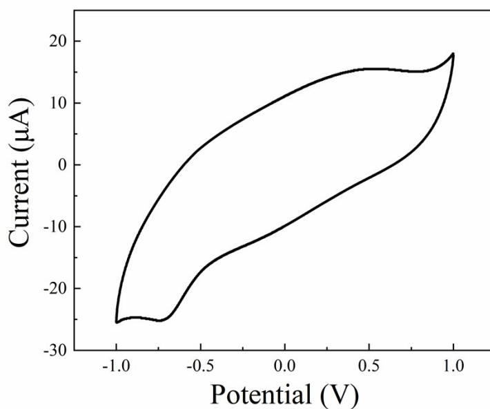
Fig. S2 CV curve of Fe 3 O 4 @Au in 0.01 M PBS (pH = 7) solution.
