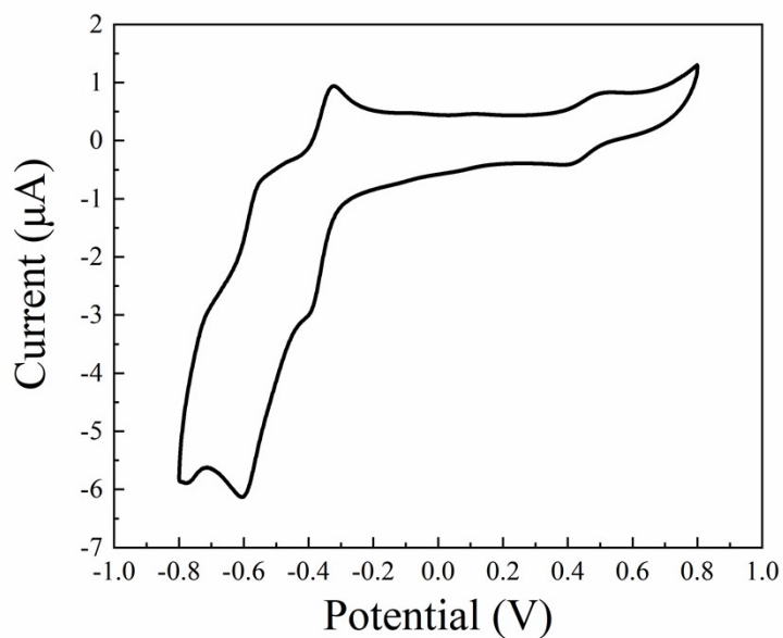
Fig. S1 CV curve of P 2 W 17 V in NaAC-AC (pH = 4) solution.
