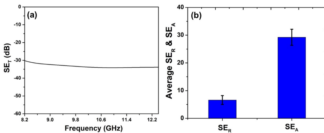
Fig. S1. SE_T and average SE_R - SE_A of 2wt. % CU/PEI composite
