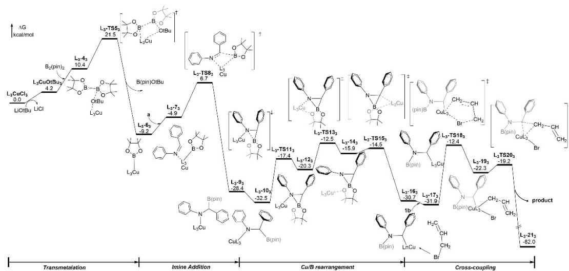
Fig. S8. Comparison of free energy profiles of solvent benzene effect on the catalytic reaction of ligand L_3 .
