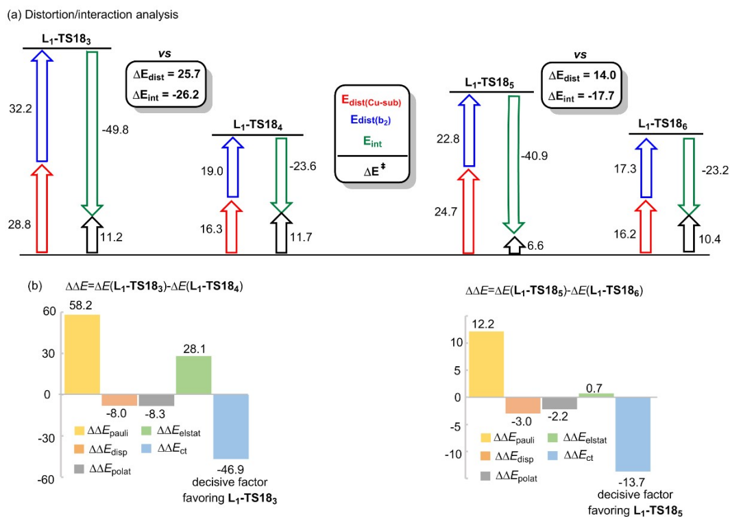
Fig. S4. DI and comparison of each energy term analysis for L 1 -TS18 3 , L 1 -TS18 4 , L 1 -TS18 5 and L 1 -TS18 6 .
