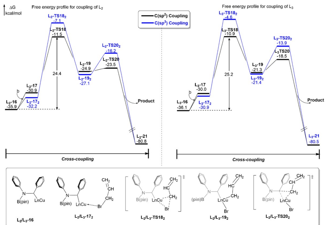
Fig. S6. Free energy profile and optimized structures of cross-coupling for L 2 and L 3 ligand.
