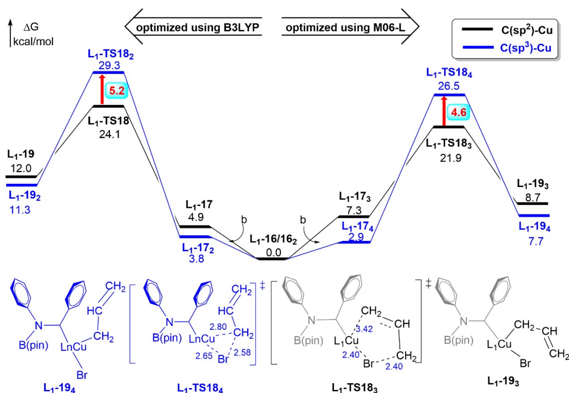
Fig. S1. Free energy profile and optimized structures of oxidation addition for L 1 .
