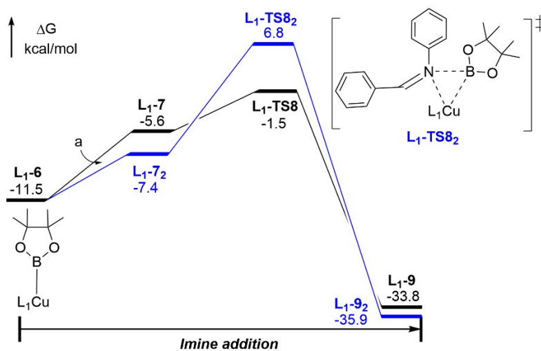
Fig. S3. Free energy profile for the generation of \alpha -borylaminoalkyl copper, along with optimized structures
