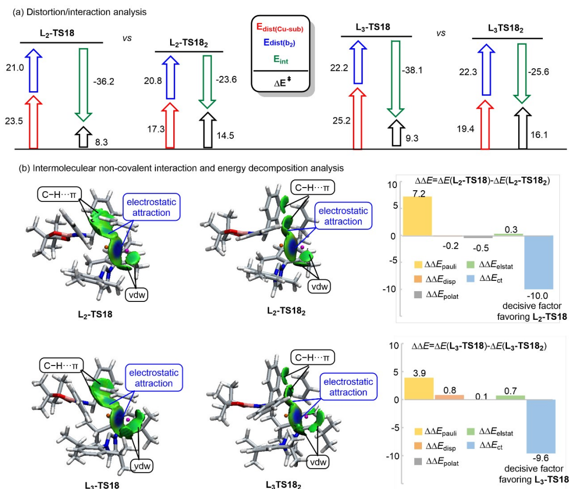
Fig. S7. (a) DI analysis. (b) NCIs and comparison of each energy term analysis for L_2\text{-TS18} , L_2\text{-TS18}_2 , L_3\text{-TS18} and L_3\text{-TS18}_2
