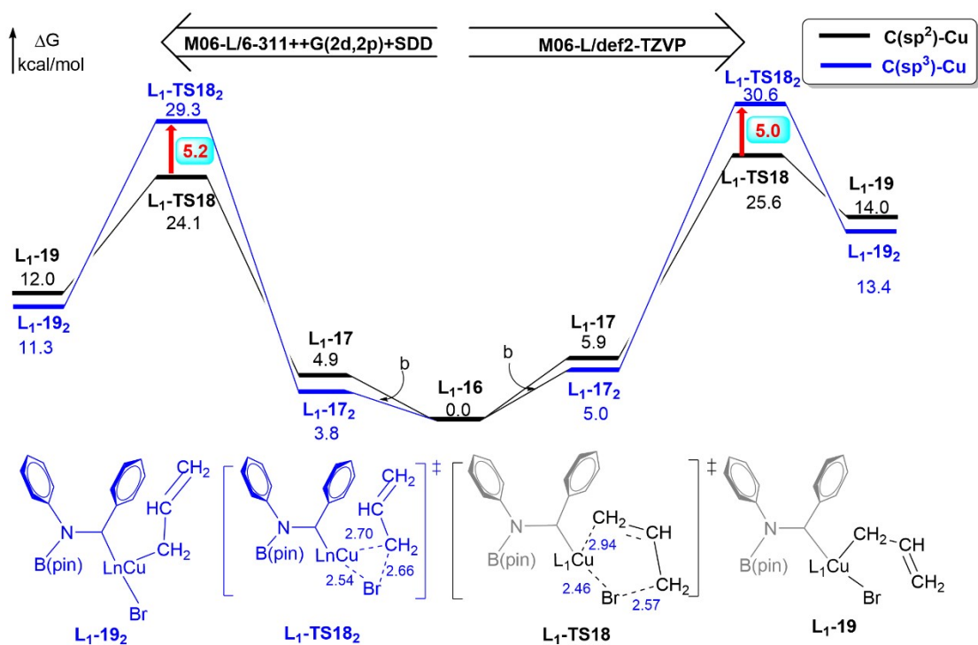
Fig. S2. Free energy profile and optimized structures of oxidation addition for L_1 .
