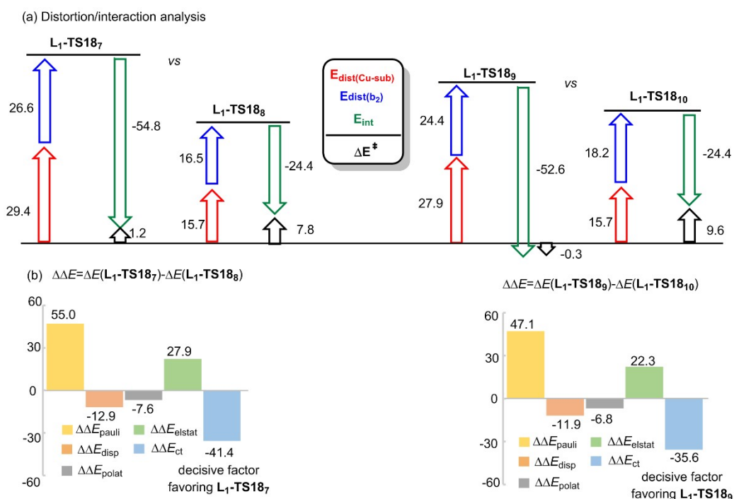
Fig. S5. DI and comparison of each energy term analysis for L 1 -TS18 7 , L 1 -TS18 8 , L 1 -TS18 9 and L 1 -TS18 10 .
