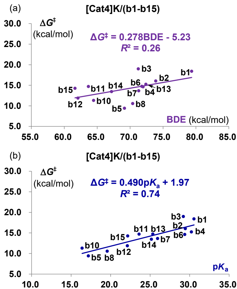
Figure S11. Activation free energy ( \Delta G^\ddagger ) versus BDE (a) and pK_a (b) in the system of [Cat4]K with b1-b15 , with exception of anomalous result for substrate b9 (not shown), potentially attributed to steric effects.
