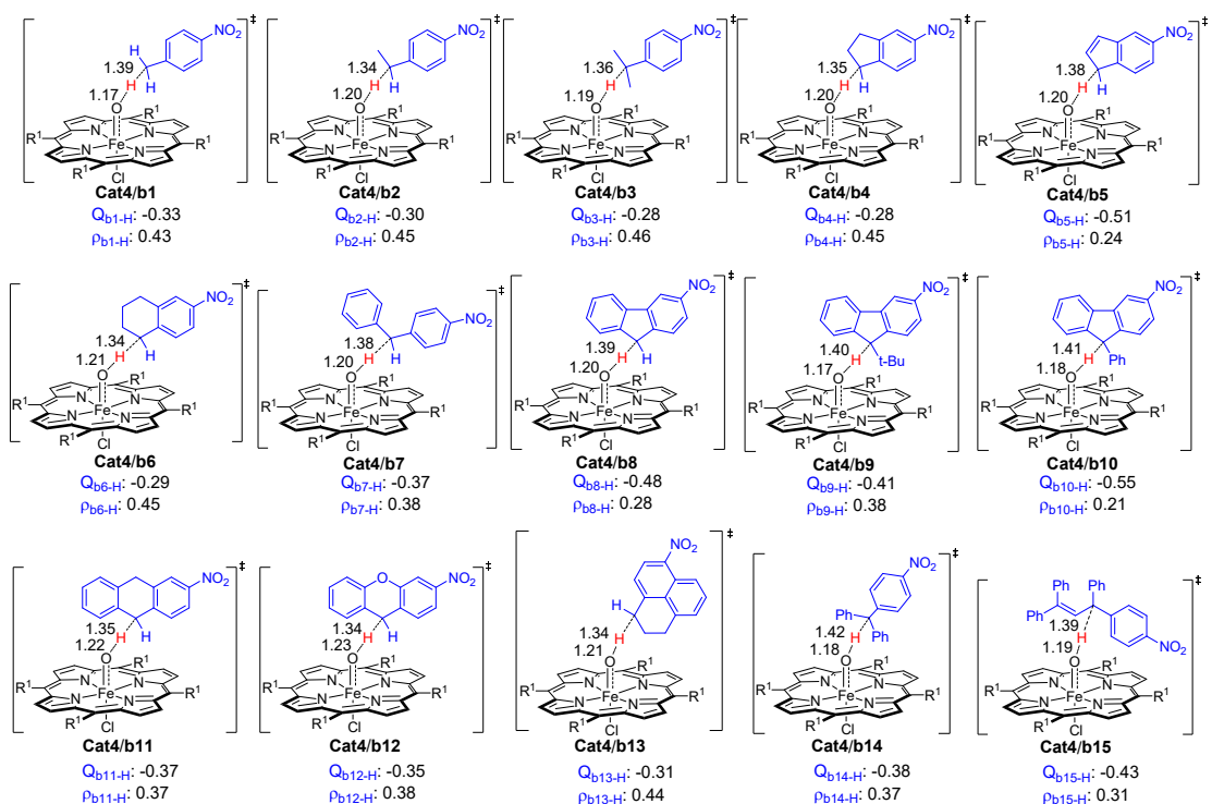
Figure S13. Geometric parameters (bond length in Å) along with NPA charges (Q) and spin densities ( \rho ) on the hydrogen-atom-abstracted substrate moiety.
