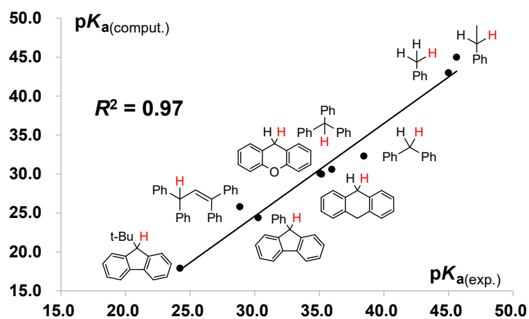
Figure S1. Plot of computational pK_a ( pK_{a(\text{comput.})} ) versus experimental pK_a ( pK_{a(\text{exp.})} ). Experimental pK_a data taken from the literature. 1
