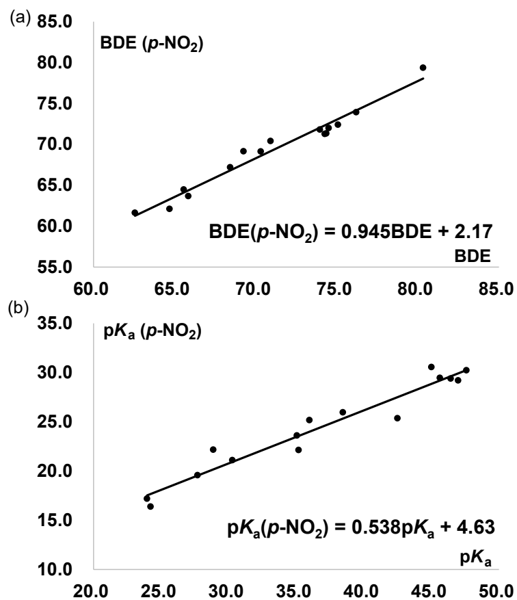
Figure S3. (a) Plot of BDE of unsubstituted substrates versus BDE of substrates bearing an electron-withdrawing group -NO_2 . (b) Plot of pK_a of unsubstituted substrates versus pK_a of substrates bearing an electron-withdrawing group -NO_2 .
