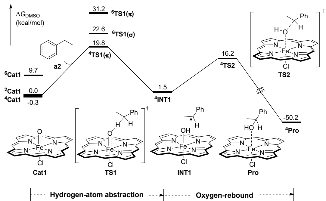
Figure S2. Gibbs free energy profiles for ethylbenzene benzylic C–H hydroxylation with Cat1 .
