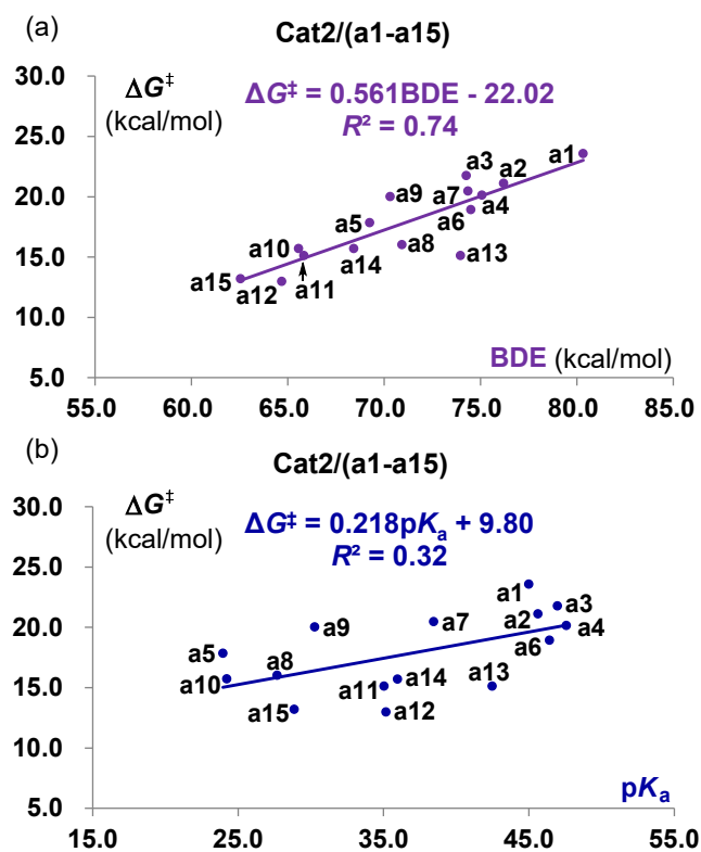
Figure S7. Activation free energy \Delta G^\ddagger versus BDE (a) and \text{p}K_a (b) in the system of Cat2 with a1-a15 .
