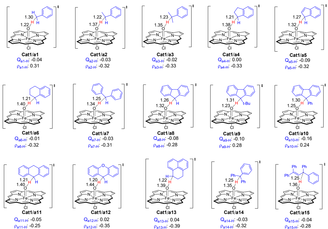
Figure S12. Geometric parameters (bond length in Å) along with NPA charges (Q) and spin densities ( \rho ) on the hydrogen-atom-abstracted substrate moiety.
