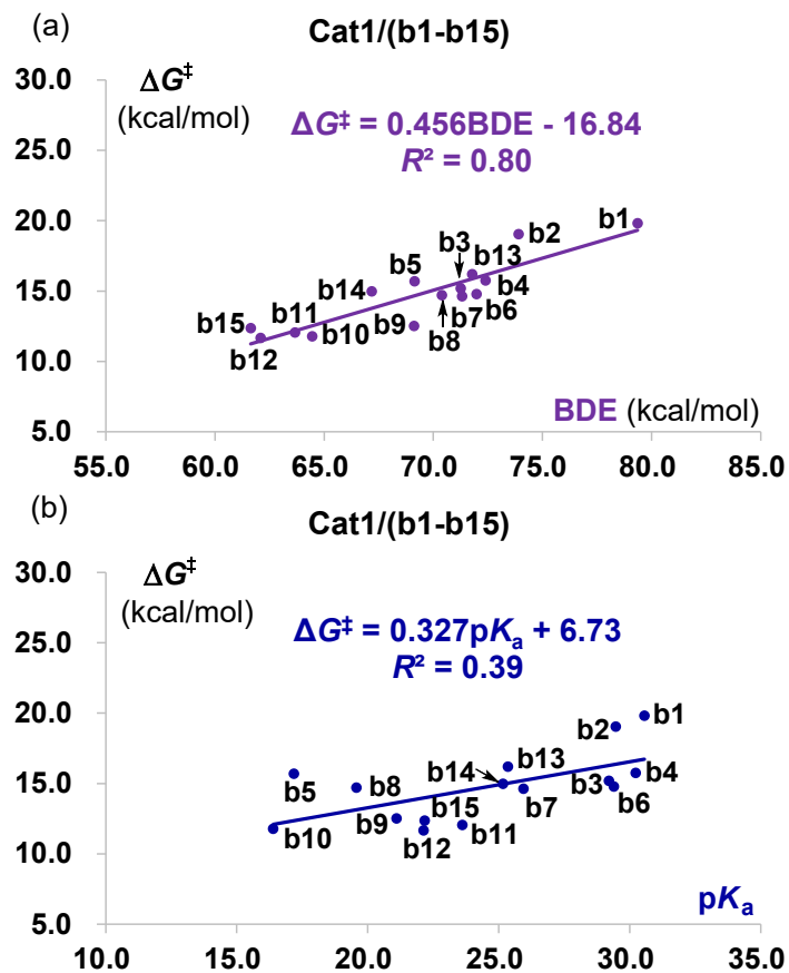
Figure S4. Activation free energy \Delta G^\ddagger versus BDE (a) and \text{p}K_a (b) in the system of Cat1 with b1-b15 .
