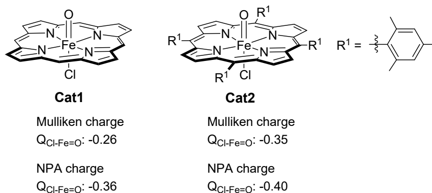
Figure S6. Mulliken charge and natural population analysis (NPA) charge (Q in e) of Cat1 and Cat2 .
