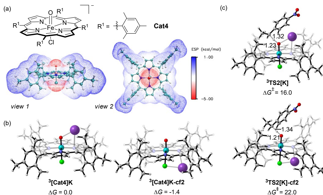
Figure S10. (a) Electrostatic potential (ESP) surface of Cat4 , optimized geometries and Gibbs free energy for {}^3[\text{Cat4}]\text{K} , {}^3[\text{Cat4}]\text{K-cf2} (b), {}^3\text{TS2}[\text{K}] and {}^3\text{TS2}[\text{K}]\text{-cf2} (c). The distances are shown in Å. The energies are shown in kcal/mol.
