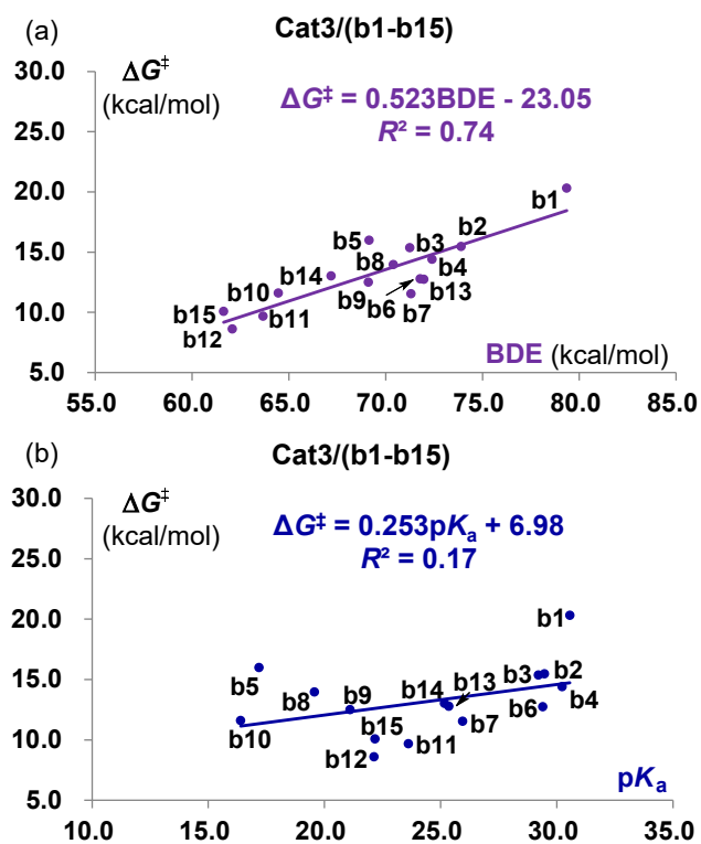
Figure S8. Activation free energy \Delta G^\ddagger versus BDE (a) and \text{p}K_a (b) in the system of Cat3 with b1-b15 .
