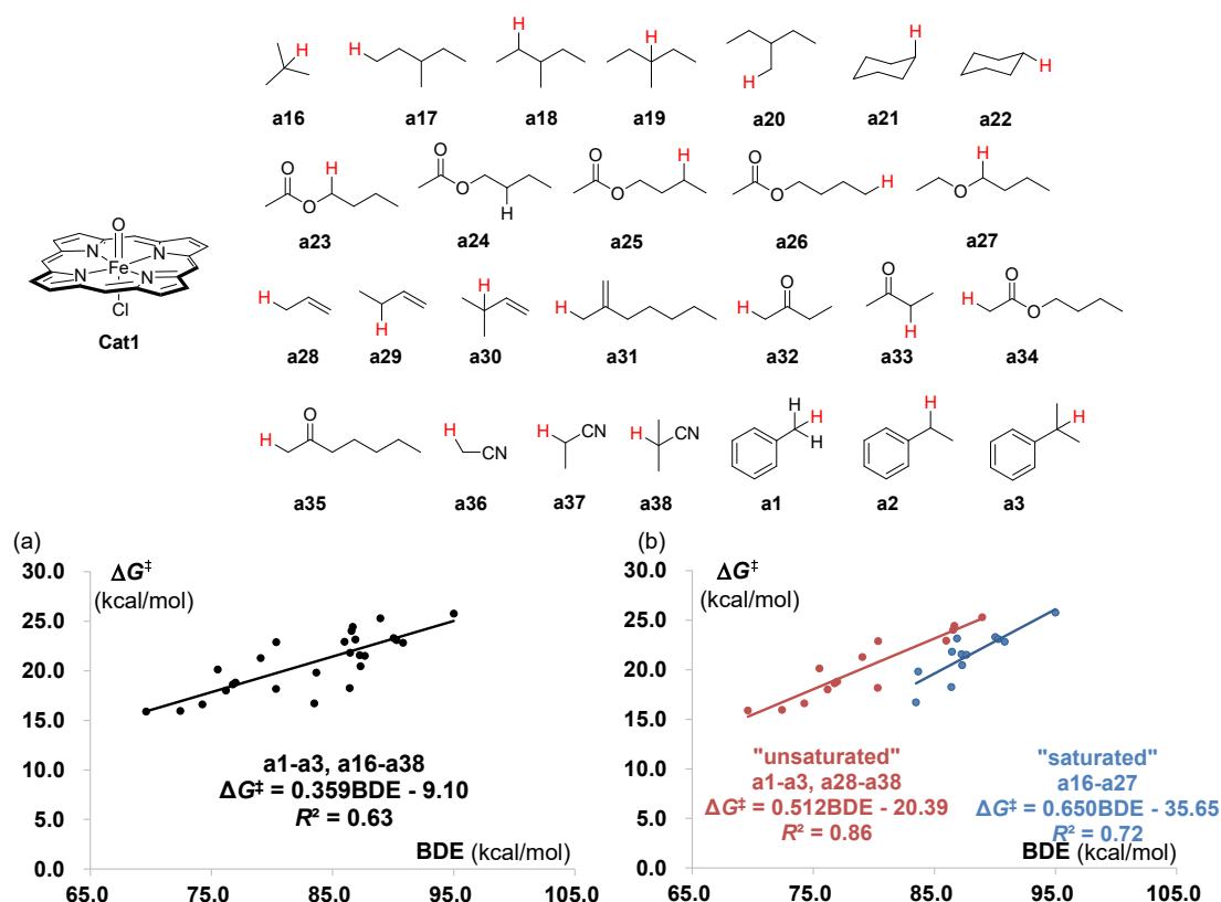
Figure S5. Activation free energy of hydroxylation by Cat1 versus BDE. (a) All the substrates investigated in this study. (b) Red dots are C–H bonds in the “unsaturated group”; blue dots are C–H bonds in the “saturated group”.
