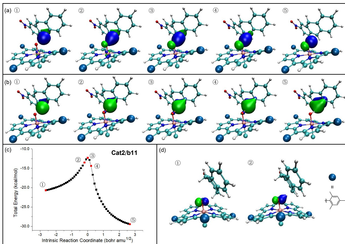
Figure S14. (a) \alpha -LMO and (b) \beta -LMO analysis along the intrinsic reaction coordinate (IRC) between Cat2 and b11 . (c) Plots of the change in electronic energies along the IRC for Cat2/b11 case. (d) \alpha -LMO of the oxo group in the Cat2/b11 case.
