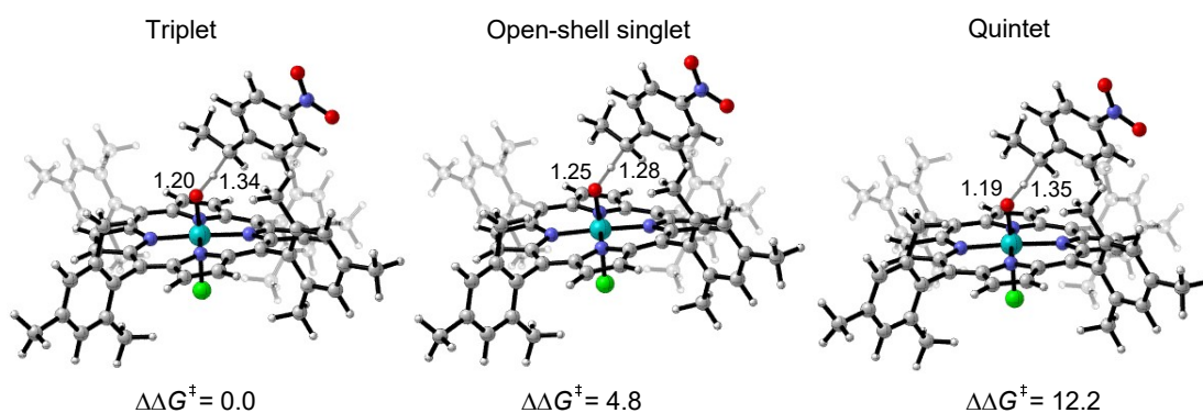
Figure S9. Optimized geometries and Gibbs free energy for transition states of Cat4 with b2 . The distances are shown in Å. The energies are shown in kcal/mol.
