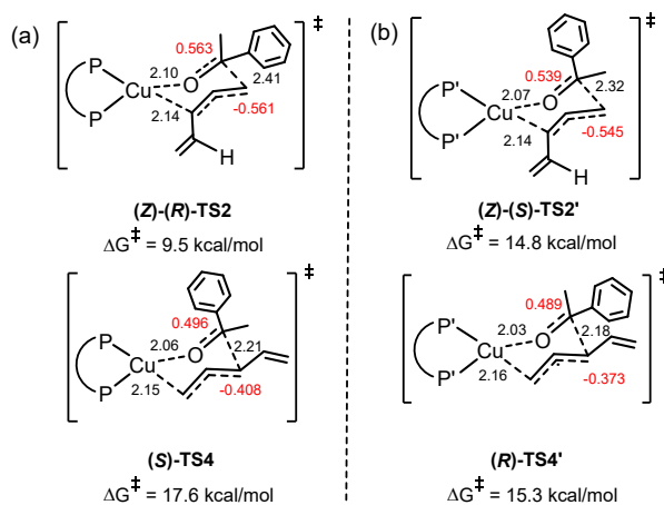
Fig. S2 NBO analyses for (a) the regioselectivity-determining transition states ( Z )-( R )- TS2 and ( S )- TS4 , as well as (b) ( Z )-( S )- TS2' and ( R )- TS4' . Energy barriers associated
