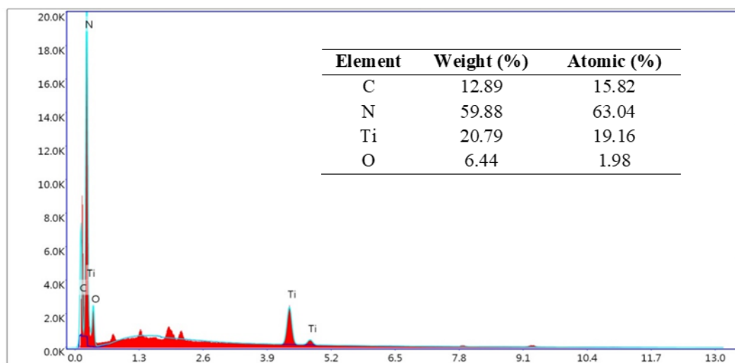
Figure S1 EDX analysis of TiO 2 /CNNS
