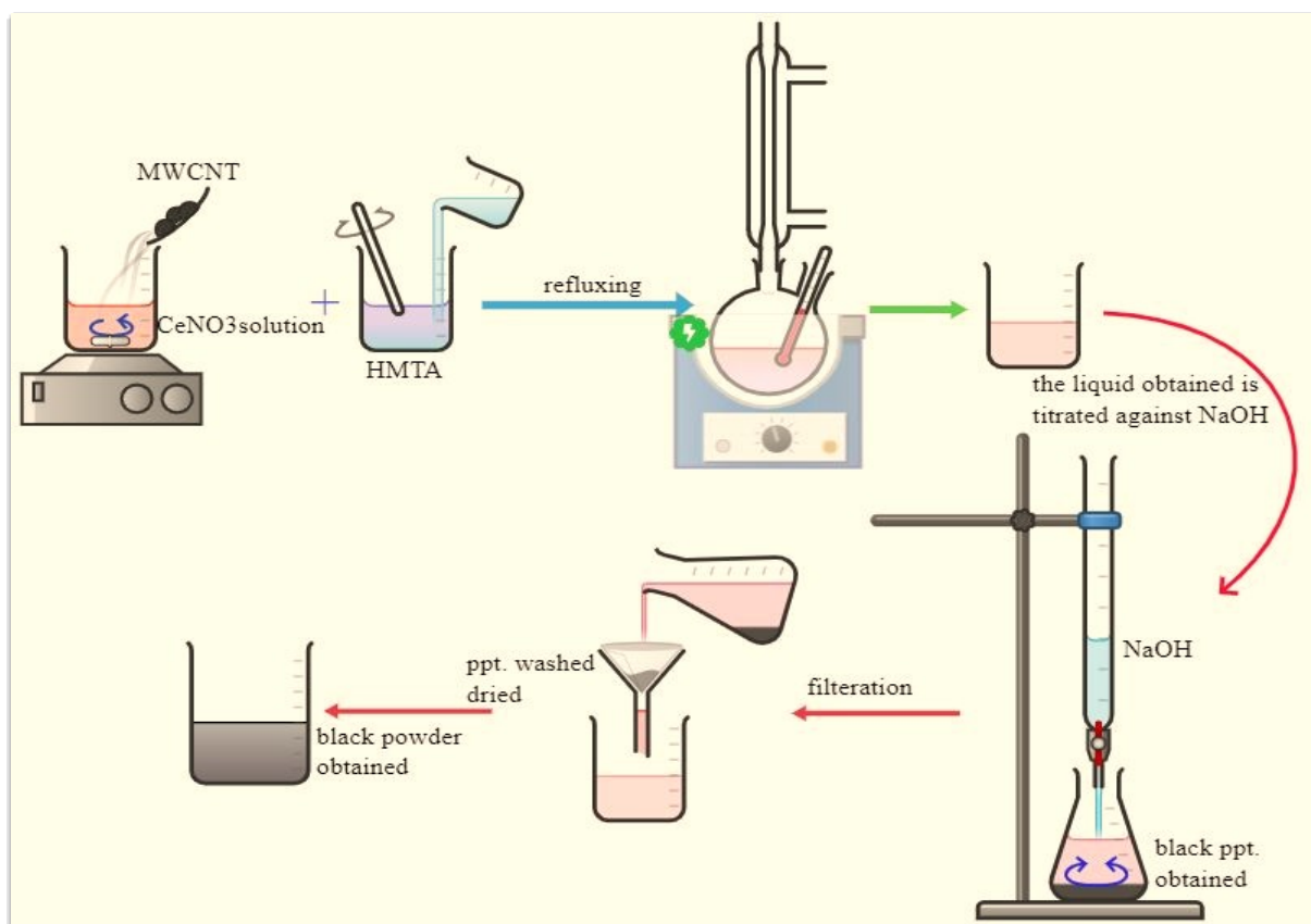
Fig. S1. Preparation of advanced hybrid CeO 2 /MWCNTs nanocomposite
