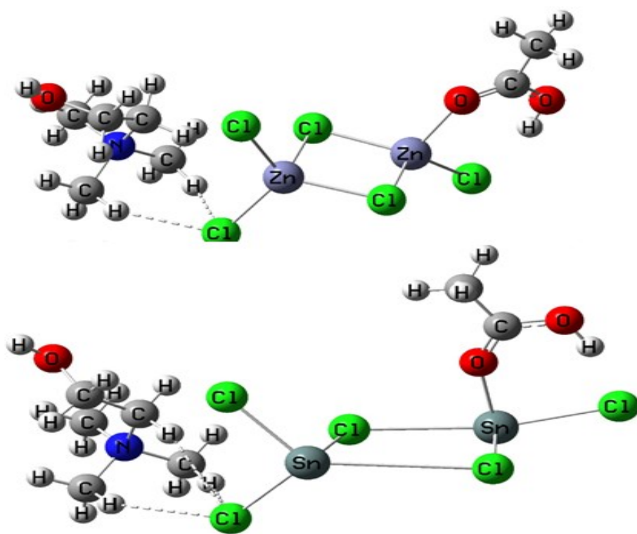
Figure S1. Optimized structures of AC adsorbed on ChCl.MCl 2 (1/2) (M = Zn and Sn).
