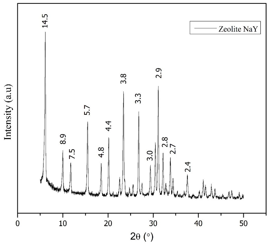
Figure S1. Diffractogram XRD of zeolite NaY with d-spacing value
