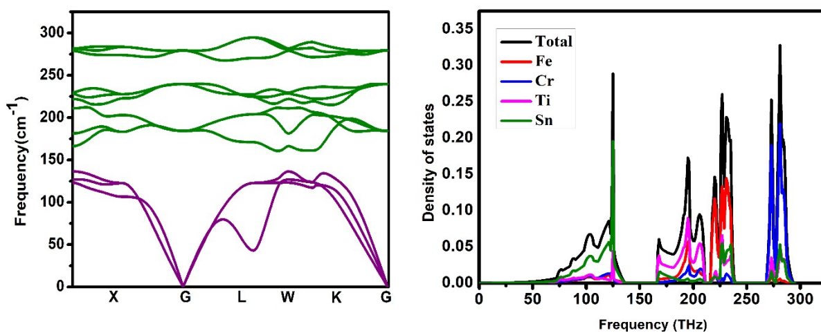
Fig 1. (a) Phonon dispersion curve and (b) total and partial density of states (DOS) of FeCrTiSn
