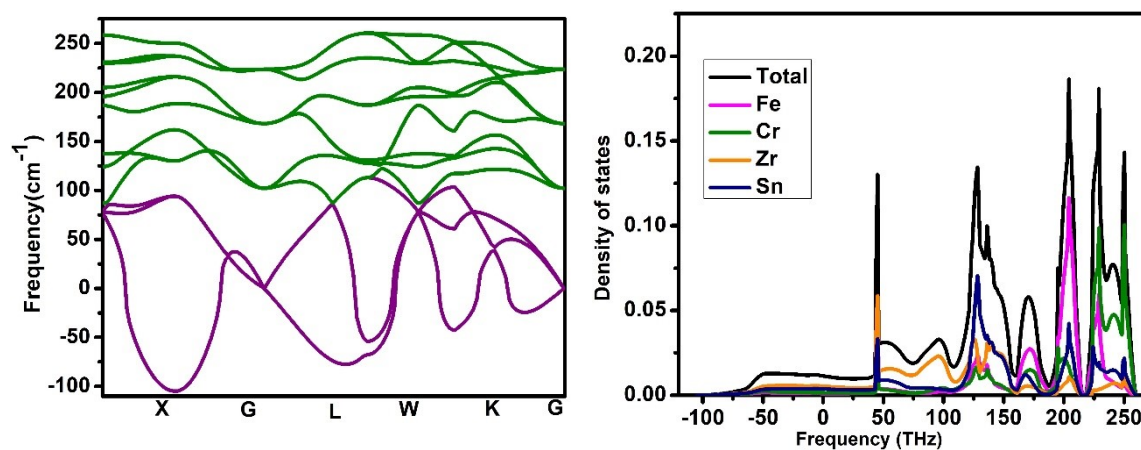
Fig 1. (b) Phonon dispersion curve and (b) total and partial density of states (DOS) of FeCrZrSn
