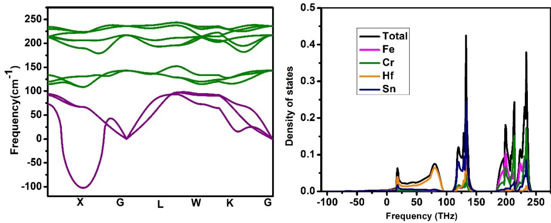
Fig 1. (c) Phonon dispersion curve and (b) total and partial density of states (DOS) of FeCrHfSn
