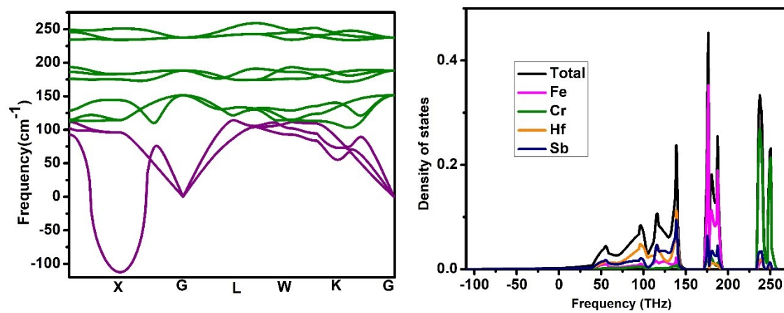
Fig 1. (e) Phonon dispersion curve and (b) total and partial density of states (DOS) of FeCrHfSb
