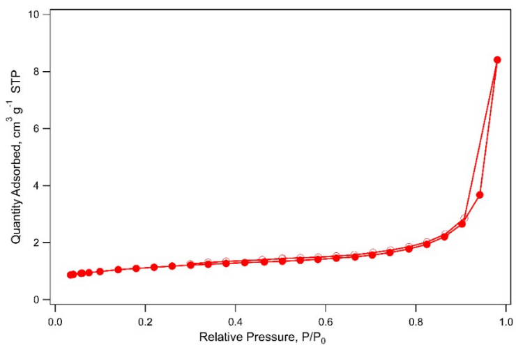
Figure S1 Nitrogen adsorption isotherm of LiHFeOFeCl
