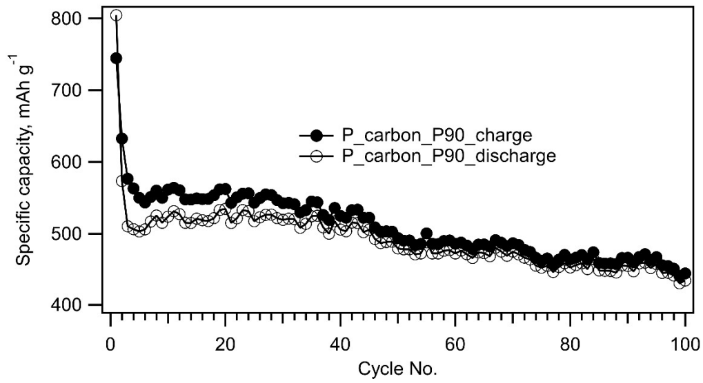
Figure S3 Galvanostatic chronopotentiometry at 0.1 C measured on the coin cell with P_carbon_P90 sulfur composite cathode
