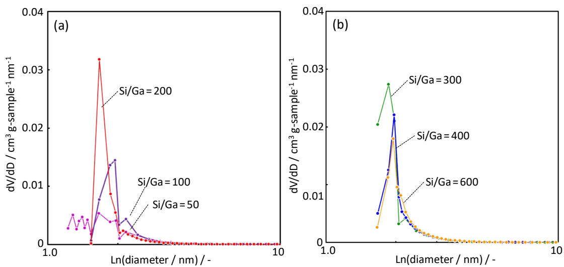
Supporting data 1 Pore size distribution in H-[Ga]-ZSM-5 catalysts.
