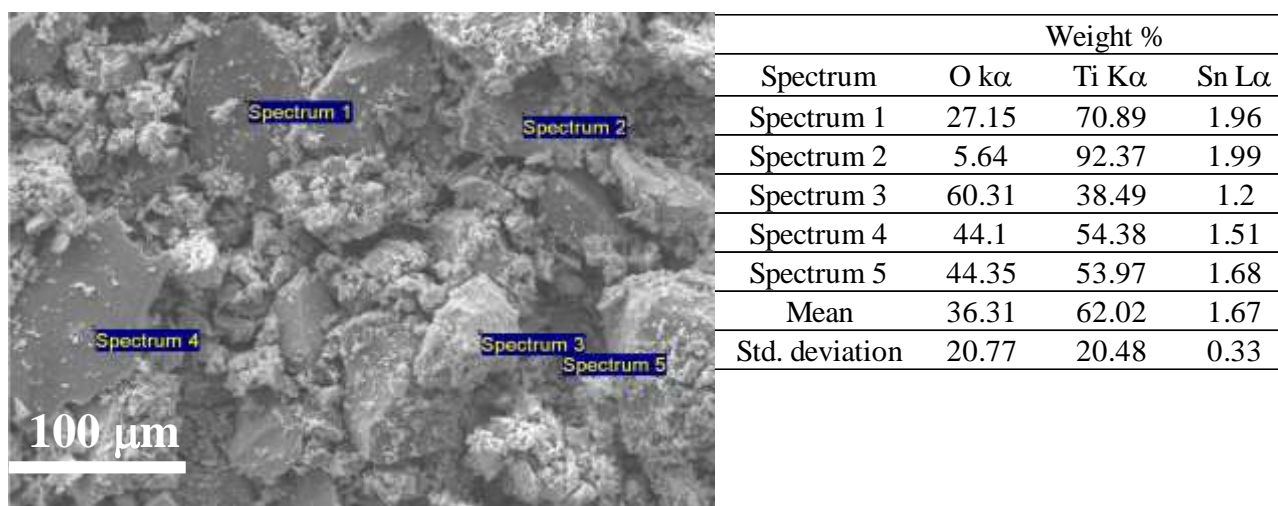
Supplementary Figure 1s. SEM analysis and punctual elemental analysis of the Sn1T photocatalyst in different areas analyzed.
