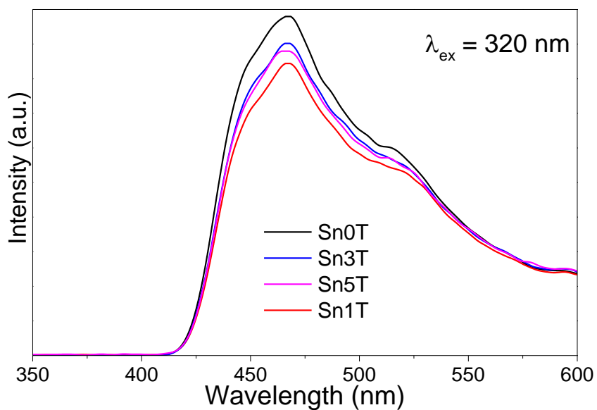
Supplementary Figure 2s. Photoluminescent spectra of photocatalyst Sn x T (x = 0, 1, 3, 5) upon excitation at 320 nm.
