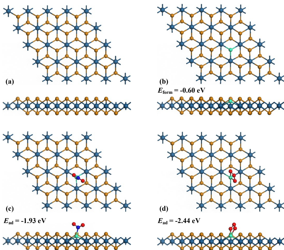
Figure S1 (a)-(b) pristine and Ni-doped 4 \times 4 \times 1 PtTe 2 monolayer, and (c)-(d) NO 2 and O 3 adsorption configurations
