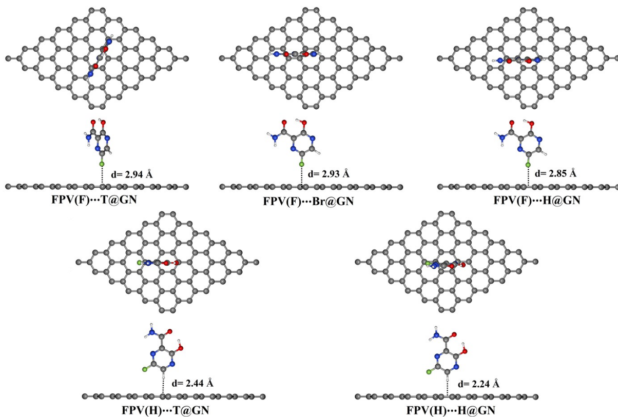
Figure S2. Relaxed structures of all FPV...GN complexes in perpendicular and parallel configurations with top and side views. The distance (d) between FPV drug and GN sheet are provided in Å.
