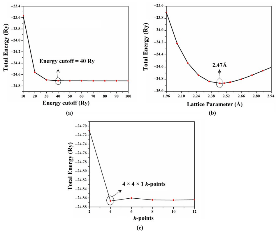
Figure S1. Convergence tests plots of the total energy with the (a) cutoff energy, (b) lattice parameter, and (c) k -point of the unit cell of GN with two C-atoms.
