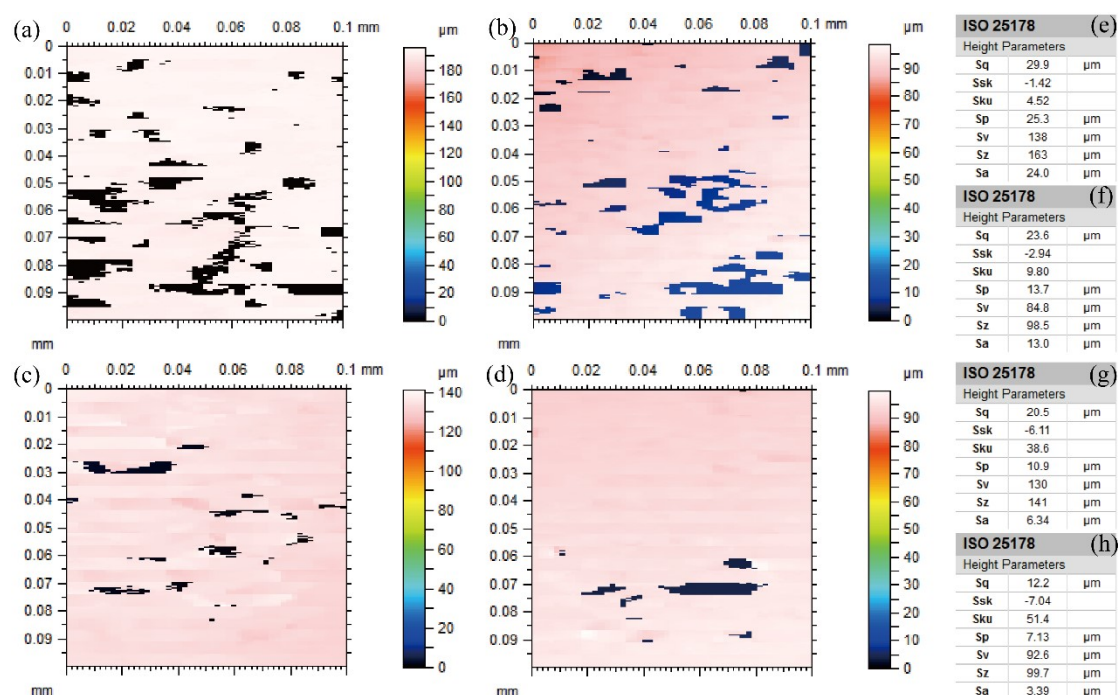
Fig. S1. (a)-(d), surface roughness topographies of samples A, A1 and samples B, B1, (e)-(h), roughness values corresponding to samples A, A1 and samples B, B1.
