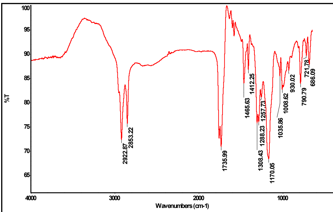
Figure S2. FT-IR spectrum of dodecyl 2-chloroactate 2b.
