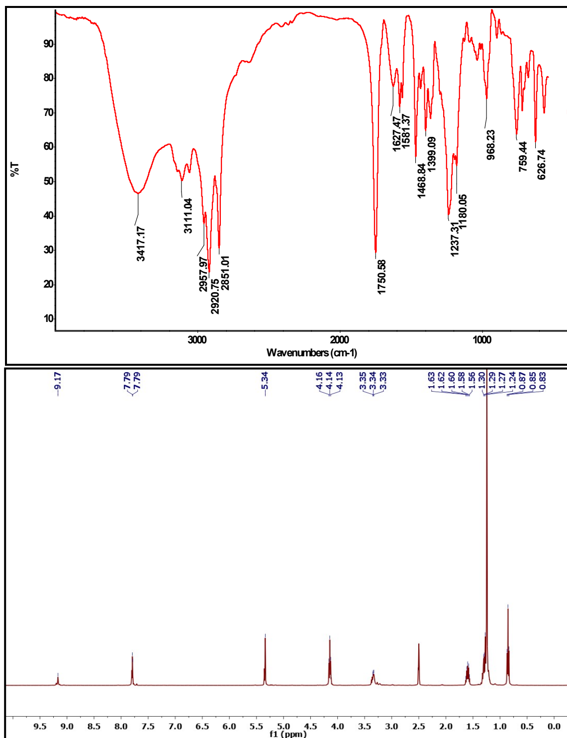
Figure S4. FT-IR and 1 H NMR (DMSO- d 6 ) spectra of the GILBS 4b.
