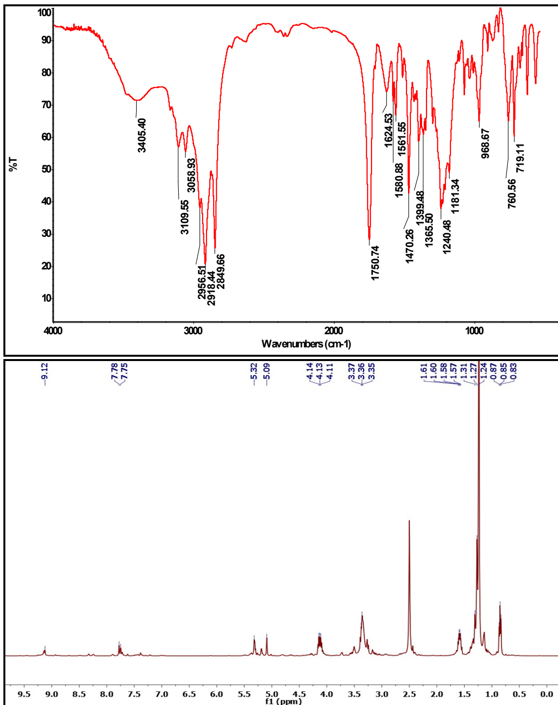
Figure S5. FT-IR and 1 H NMR (DMSO- d 6 ) spectra of the GILBS 4c.
