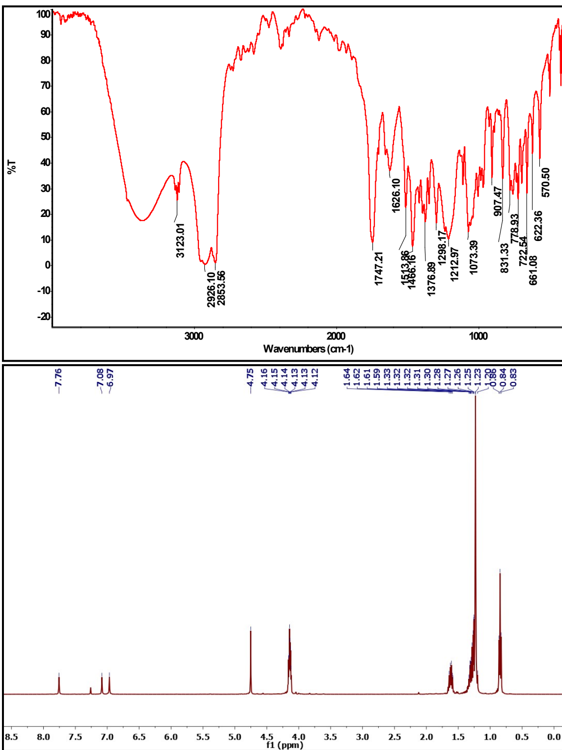
Figure S3. FT-IR and 1 H NMR spectra (CDCl 3 ) of alkyl imidazole derivative 3a.
