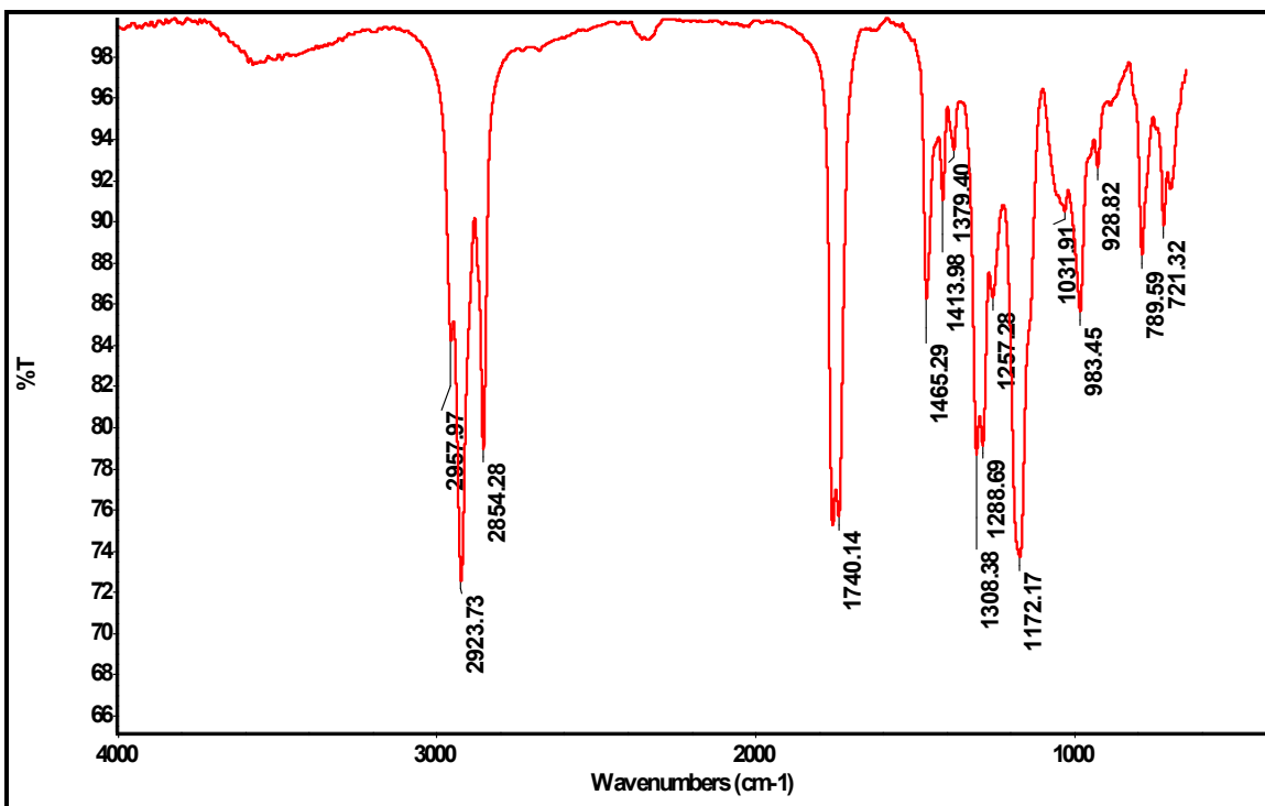
Figure S1. FT-IR spectrum of decyl 2-chloroactate 2a.
