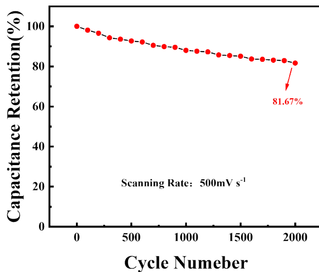
Fig.1S Cyclic stability testing of 2F-CMSC fabricated by EDR technique
