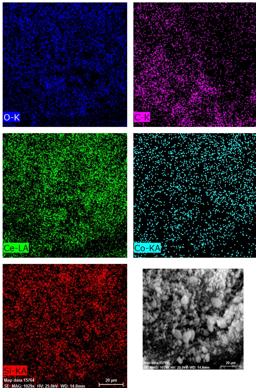
Fig. S2. FESEM/Map data of NC Catalyst.
