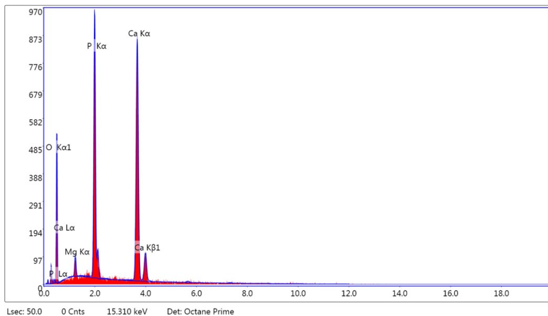
Figure S_1: Pictorial view of elemental analysis by EDX for drug loaded sample
