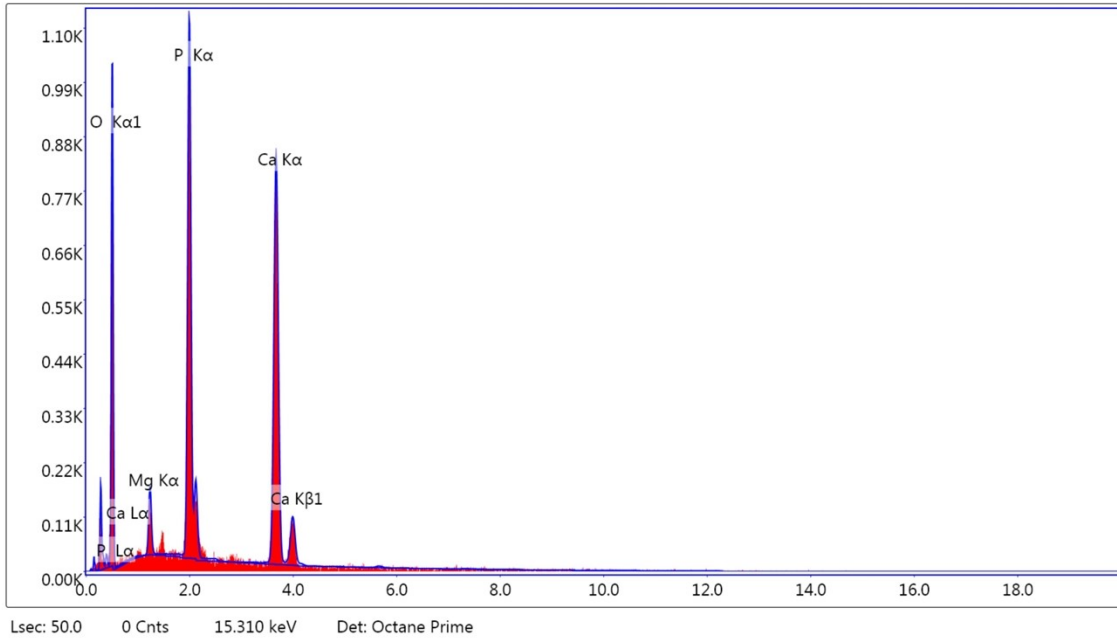
Figure S_2: Pictorial view of elemental analysis by EDX after drug release
