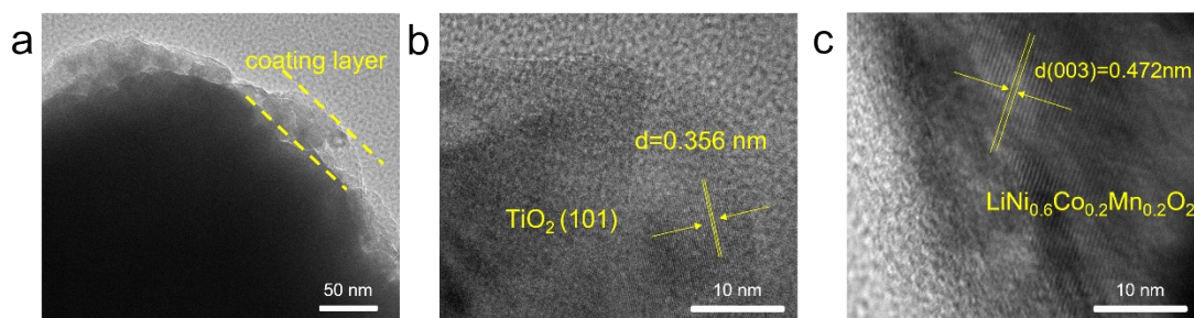
Figure S1. (a-c) HRTEM images of NCM622/TF-0.2%.
