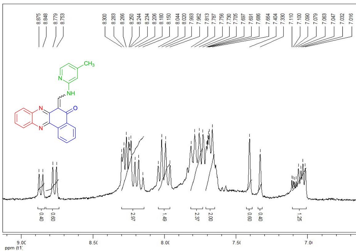
1 H-NMR spectrum of compound 6c (300 MHz, DMSO- d 6 )
