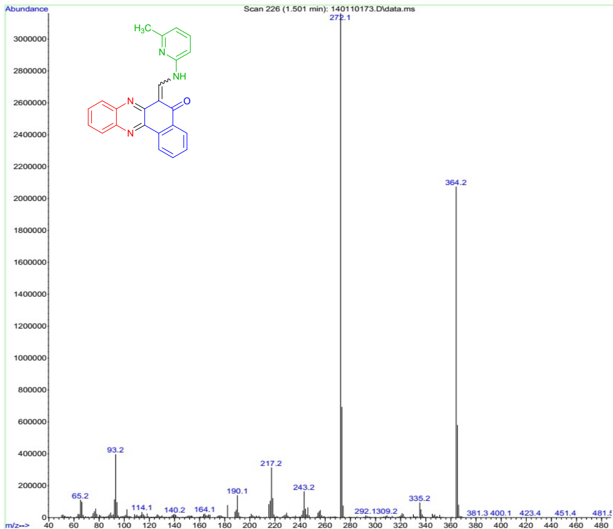
Mass spectrum of compound 6a
