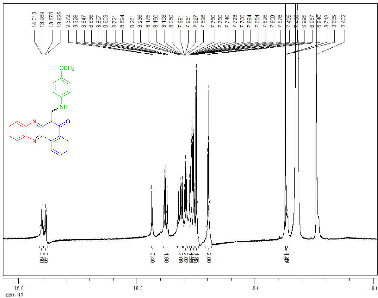
1 H-NMR spectrum of compound 6i (300 MHz, DMSO- d 6 )
