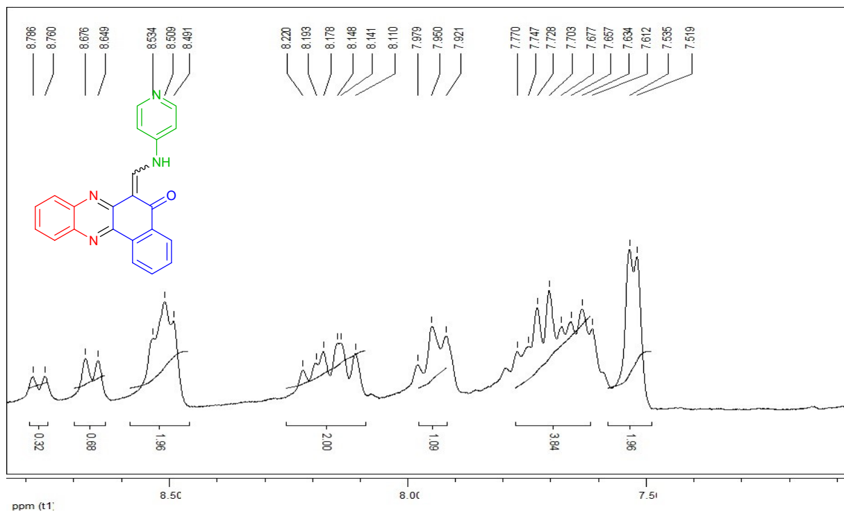
1 H-NMR spectrum of compound 6e (300 MHz, DMSO- d 6 )
