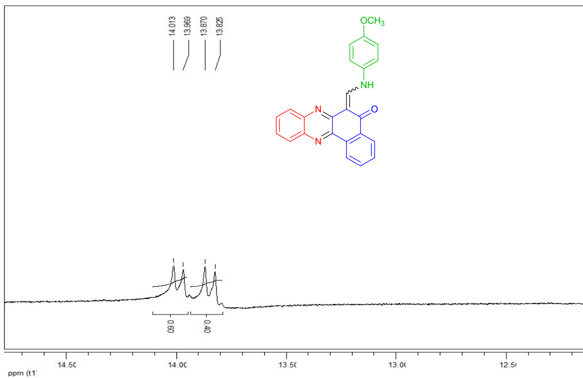
13 C-NMR spectrum of compound 6i (300 MHz, DMSO- d 6 )
