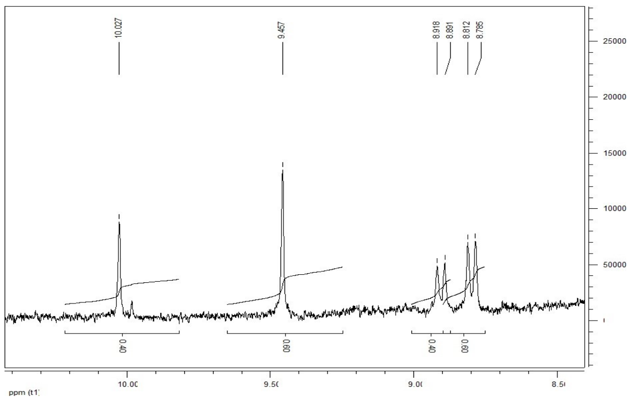
1 H-NMR spectrum of compound 6a (300 MHz, DMSO- d 6 + D 2 O)
