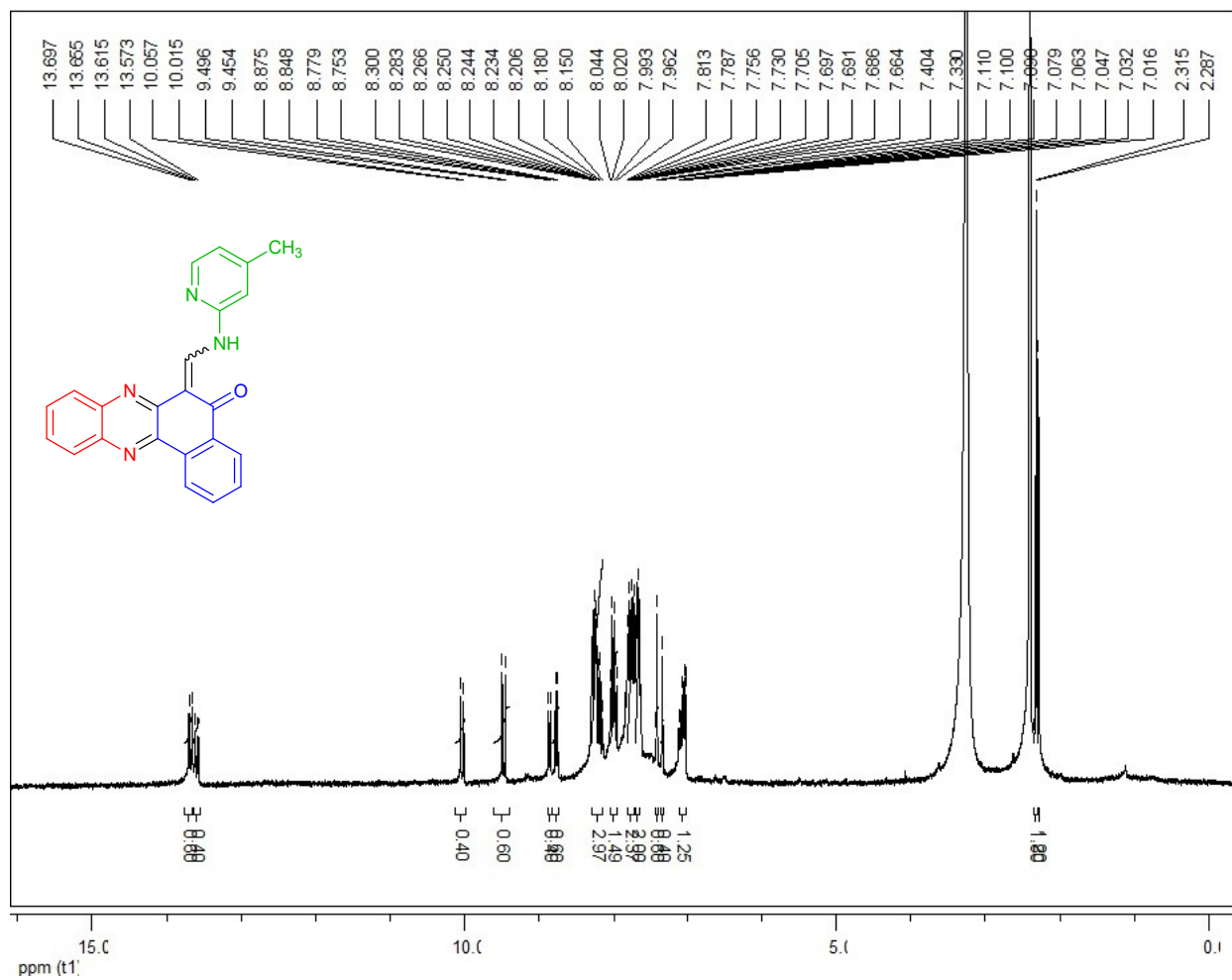
1 H-NMR spectrum of compound 6c (300 MHz, DMSO- d 6 )
