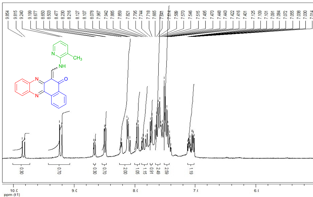
1 H-NMR spectrum of compound 6b (300 MHz, DMSO- d 6 )
