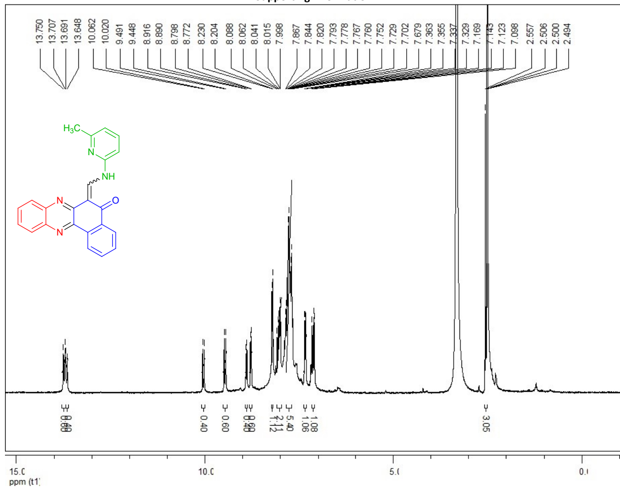
1 H-NMR spectrum of compound 6a (300 MHz, DMSO- d 6 )
