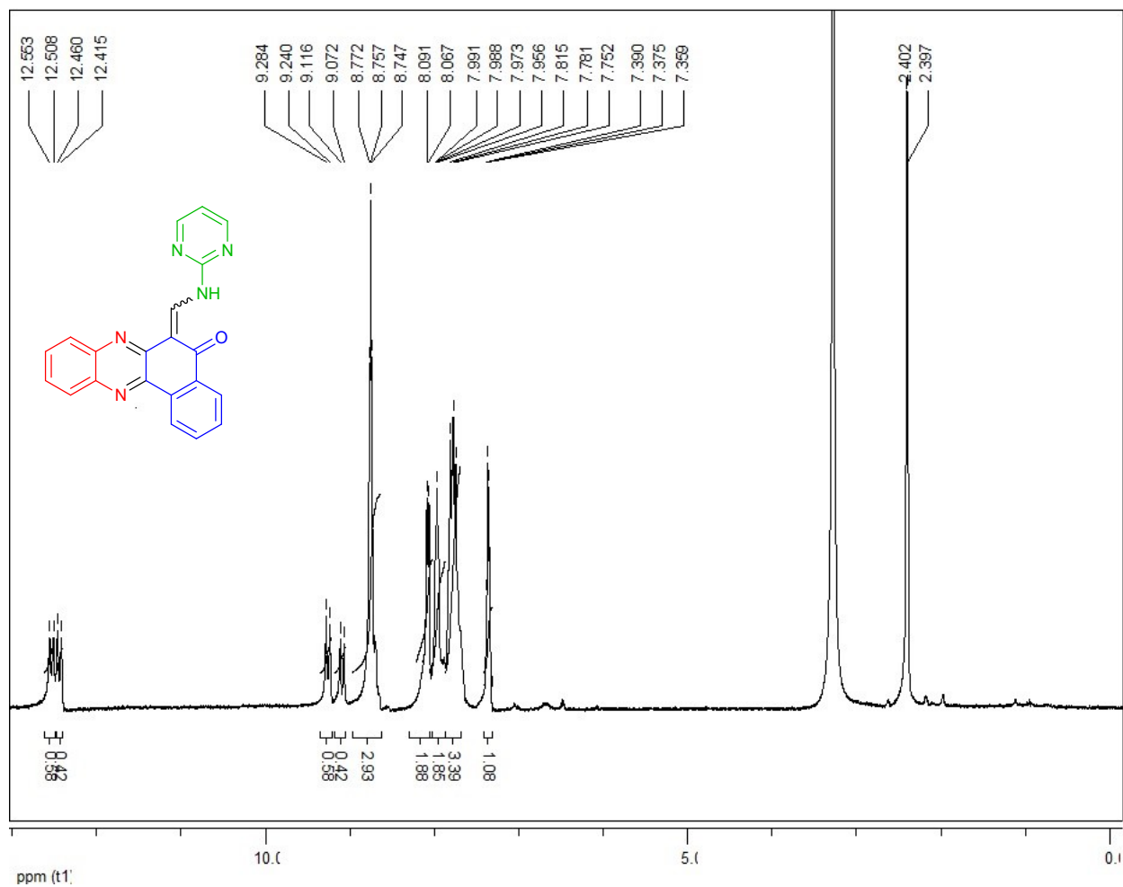
^1\text{H-NMR} spectrum of compound 6f (300 MHz, \text{DMSO-d}_6 )
