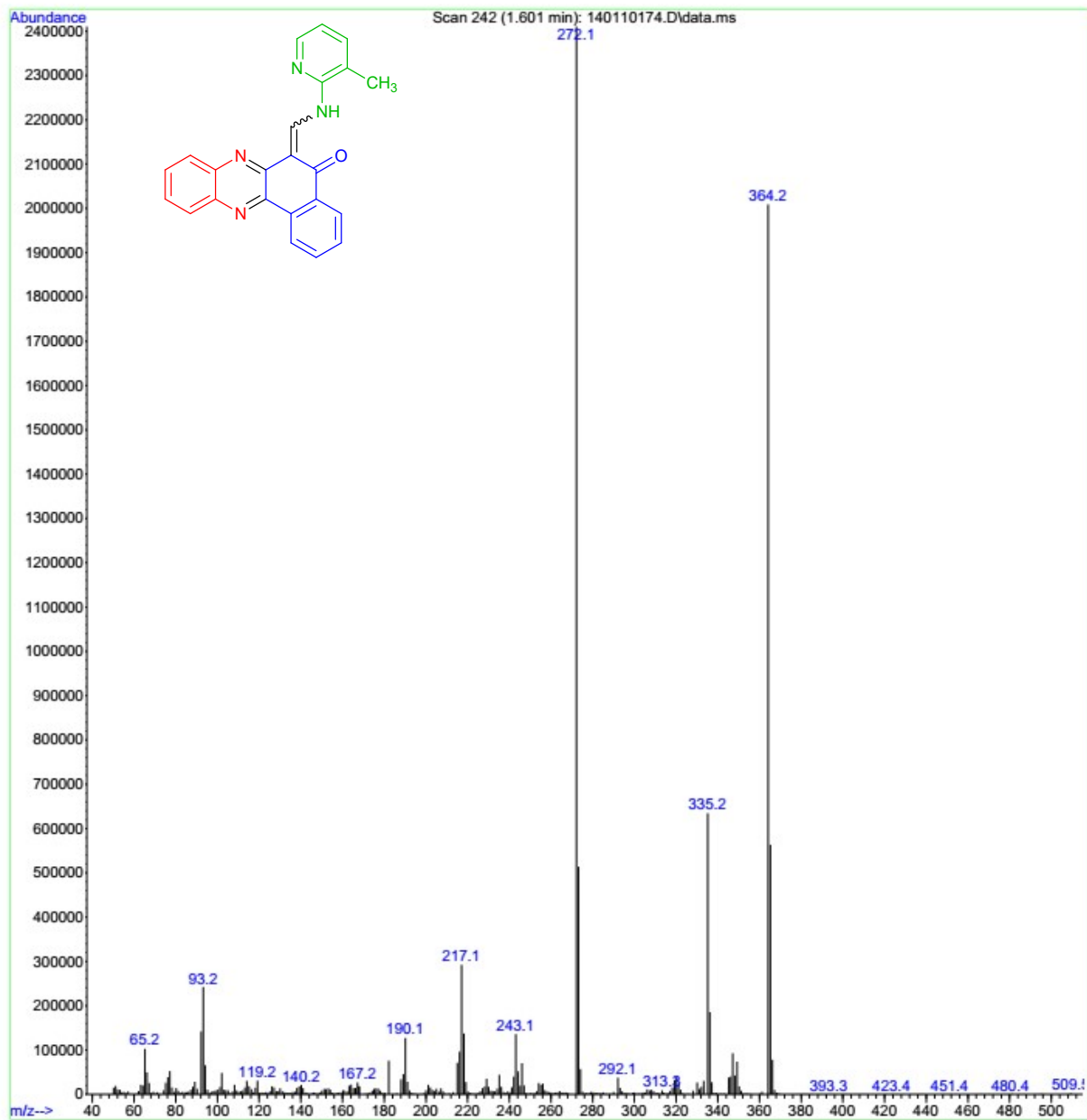
Mass spectrum of compound 6b
