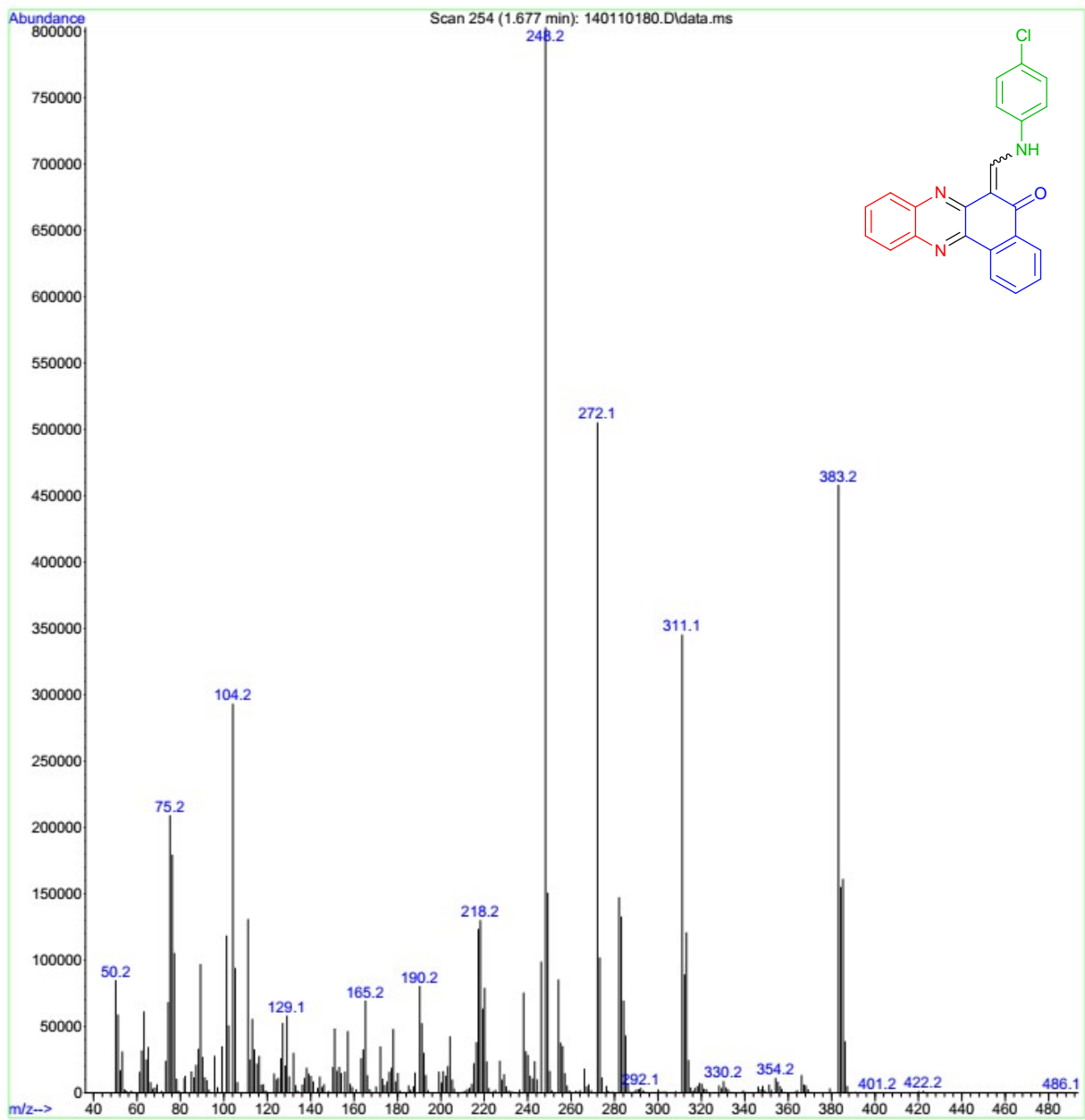
Mass spectrum of compound 6g
