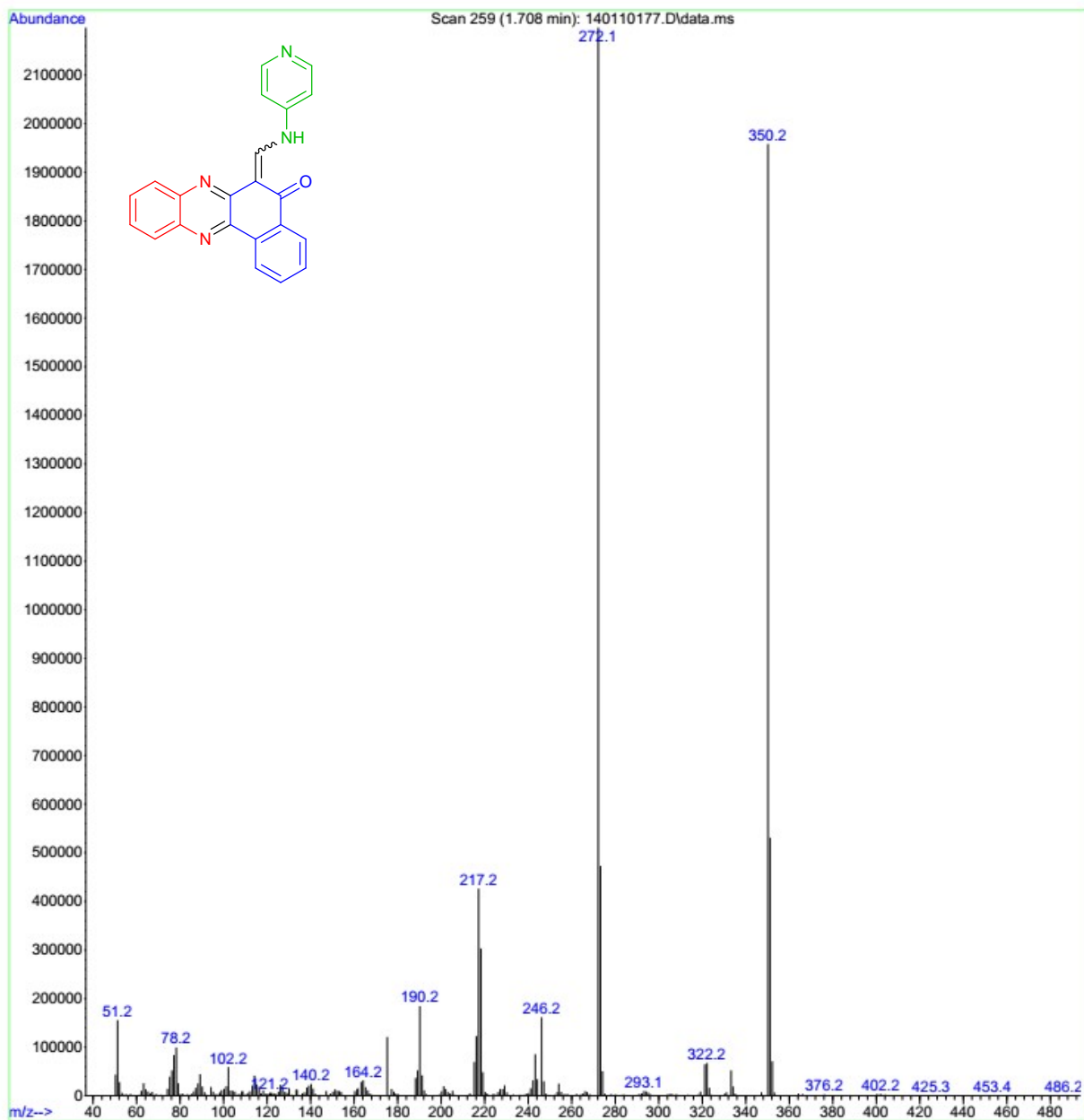
Mass spectrum of compound 6e
