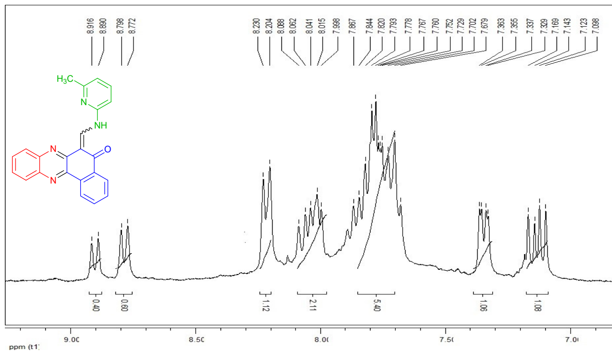
1 H-NMR spectrum of compound 6a (300 MHz, DMSO- d 6 )
