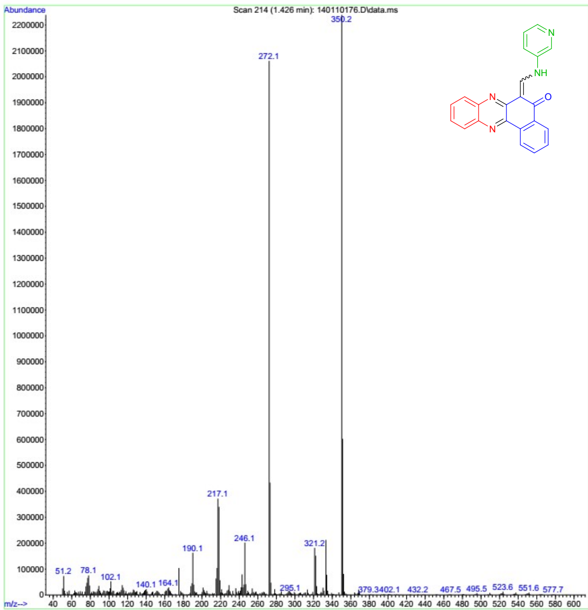
Mass spectrum of compound 6d
