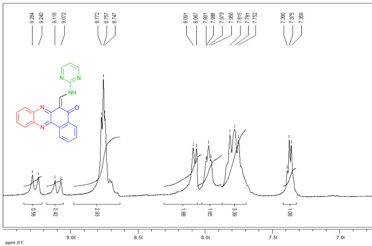
1 H-NMR spectrum of compound 6f (300 MHz, DMSO- d 6 )
