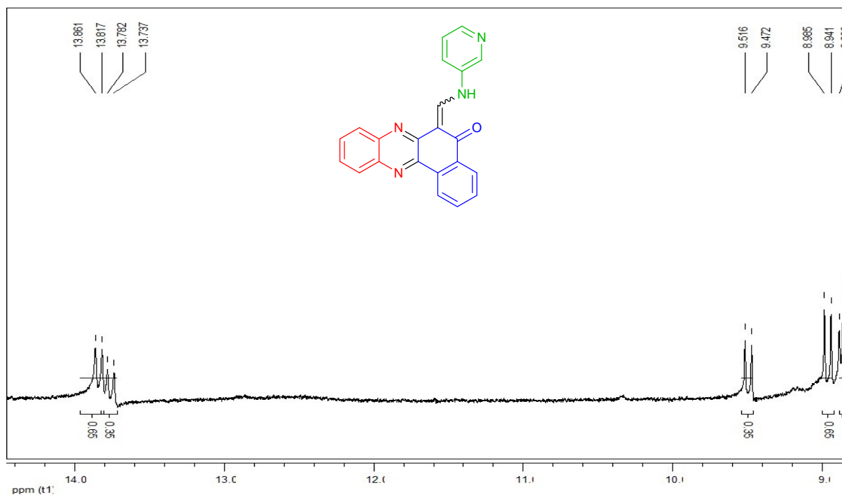
1 H-NMR spectrum of compound 6d (300 MHz, DMSO- d 6 )
