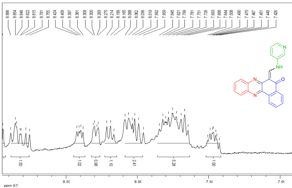
1 H-NMR spectrum of compound 6d (300 MHz, DMSO- d 6 )
