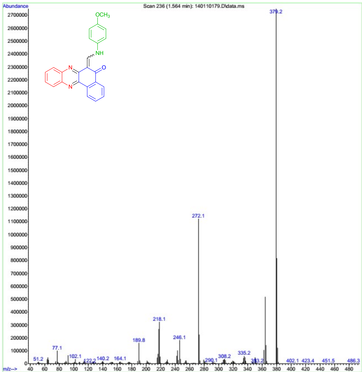
Mass spectrum of compound 6i
