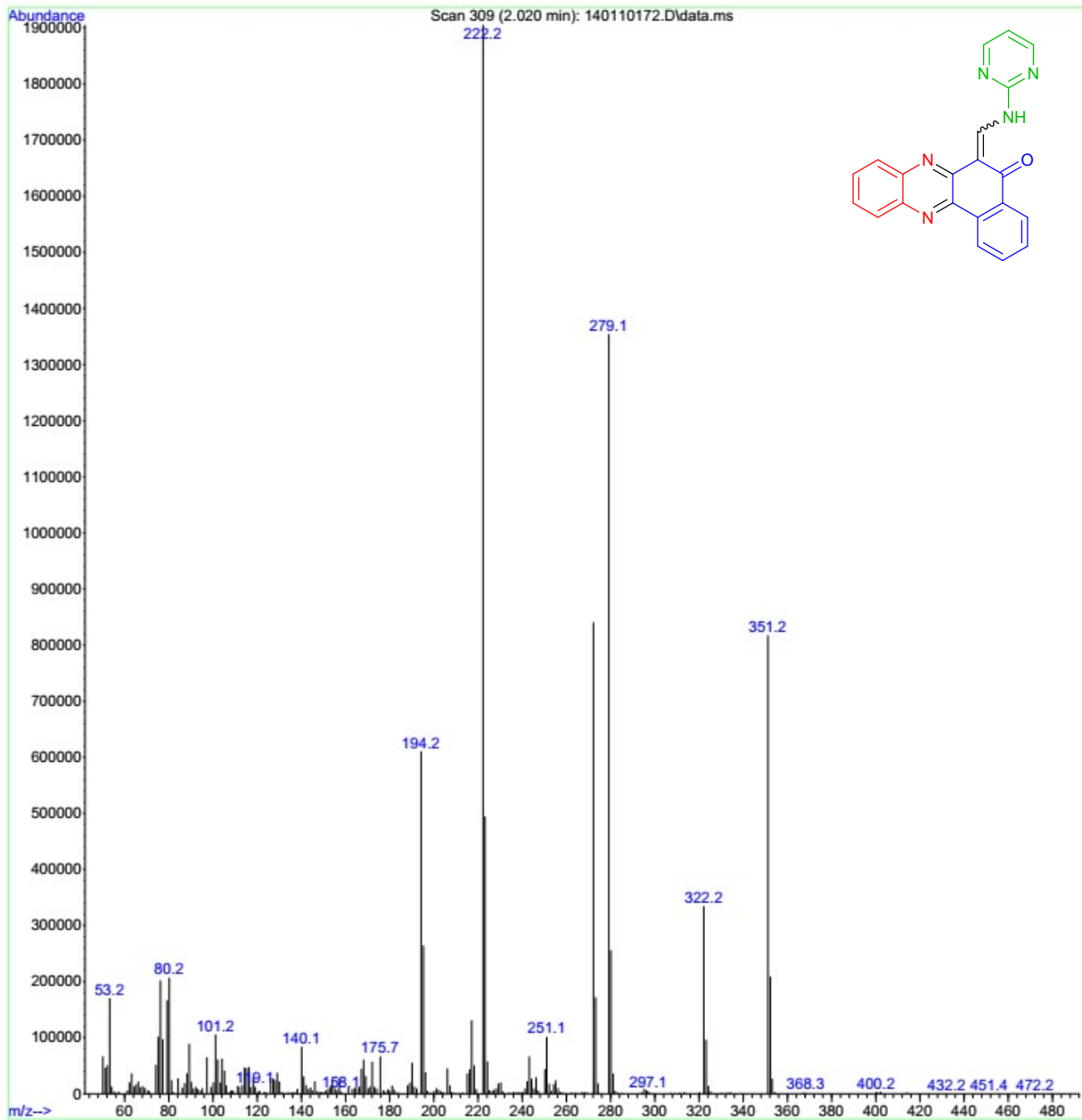
Mass spectrum of compound 6f
