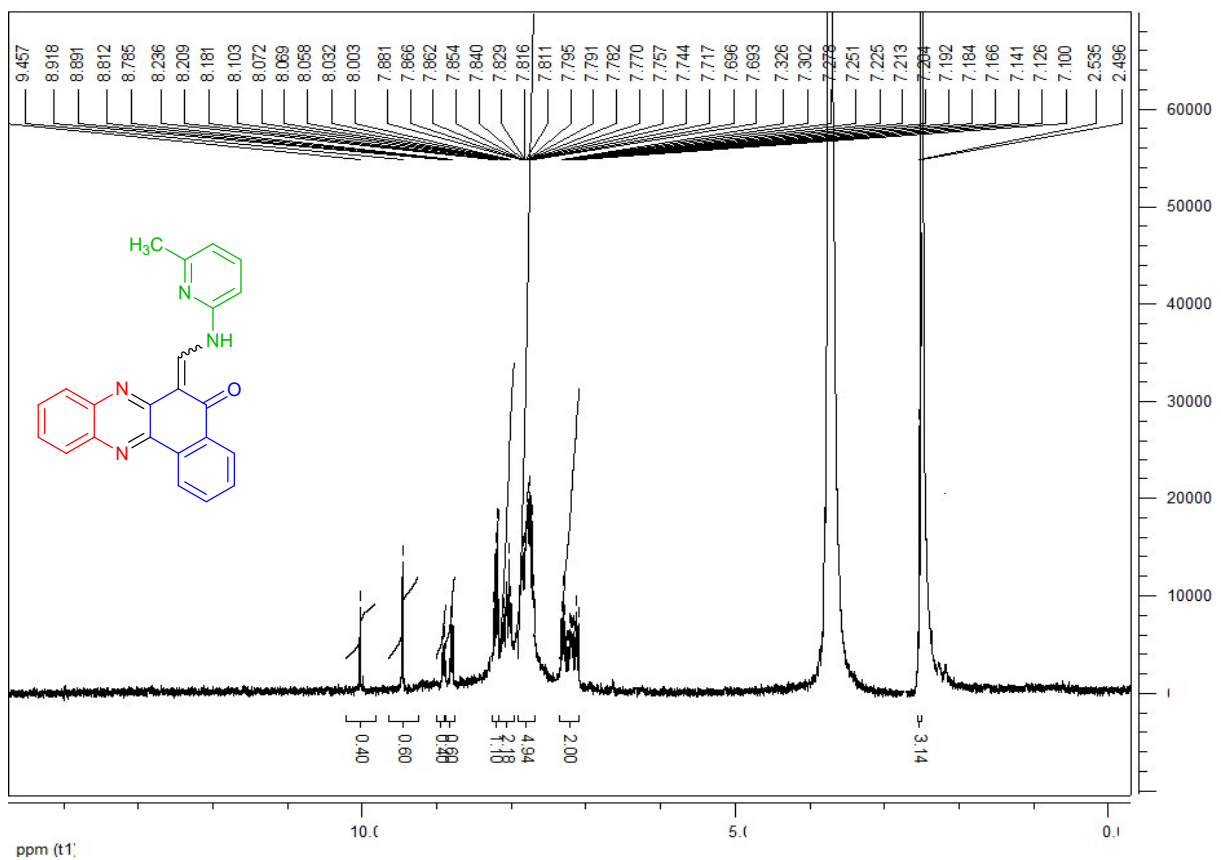
1 H-NMR spectrum of compound 6a (300 MHz, DMSO-d 6 + D 2 O)
