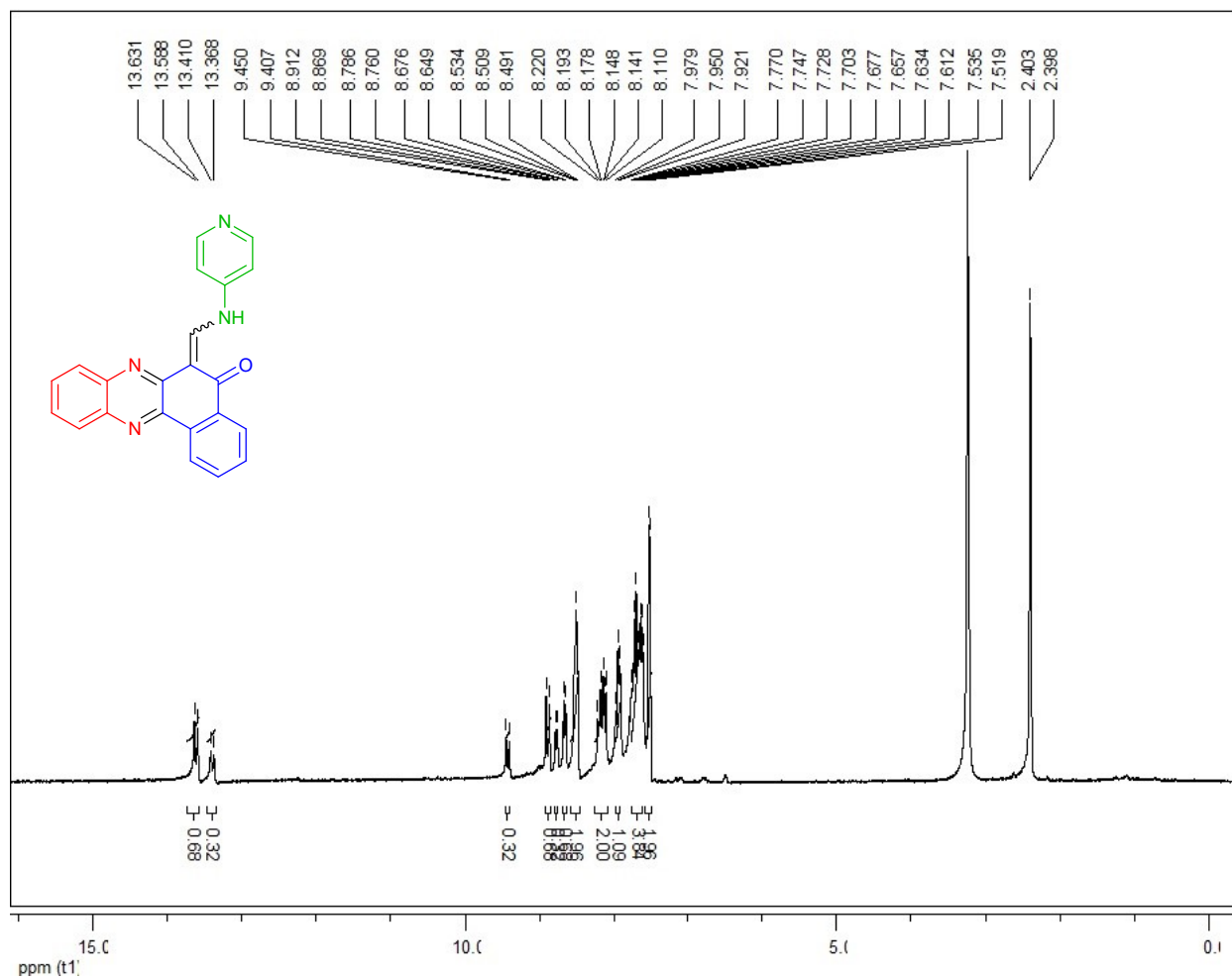
1 H-NMR spectrum of compound 6e (300 MHz, DMSO- d 6 )
