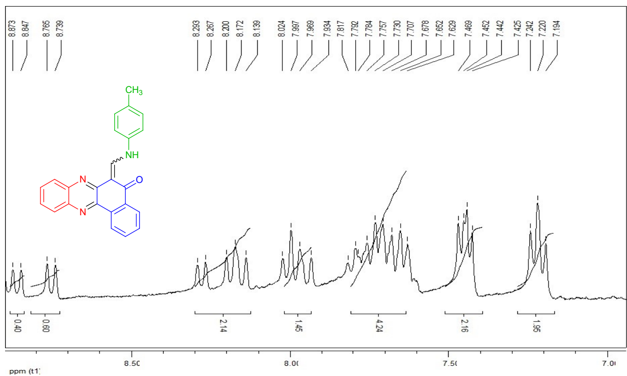
1 H-NMR spectrum of compound 6h (300 MHz, DMSO- d 6 )
