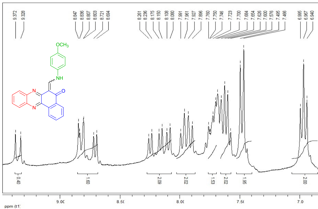
1 H-NMR spectrum of compound 6i (300 MHz, DMSO- d 6 )
