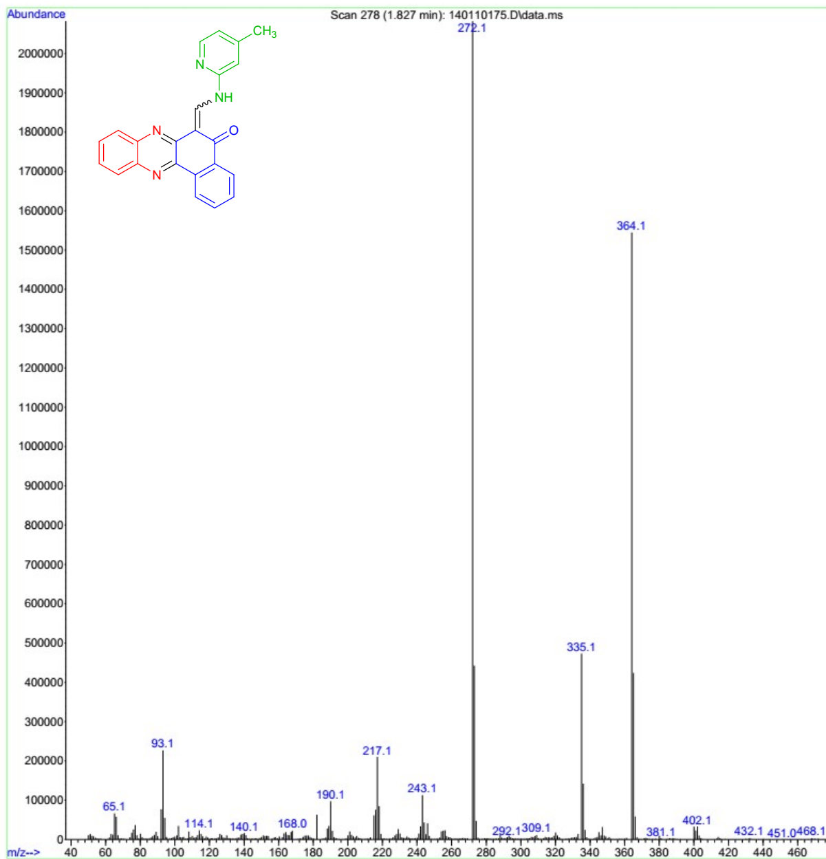
Mass spectrum of compound 6c
