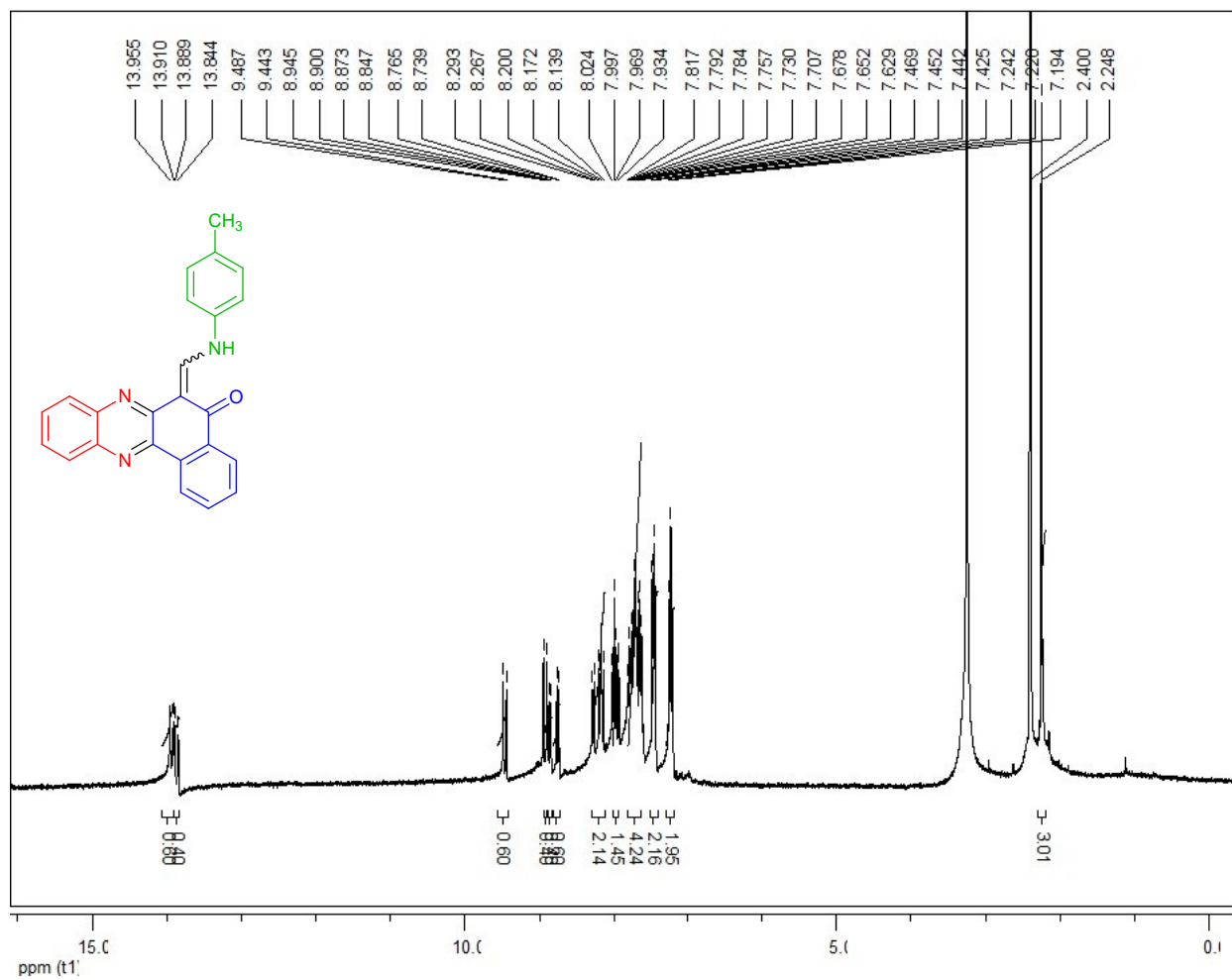
1 H-NMR spectrum of compound 6h (300 MHz, DMSO- d 6 )
