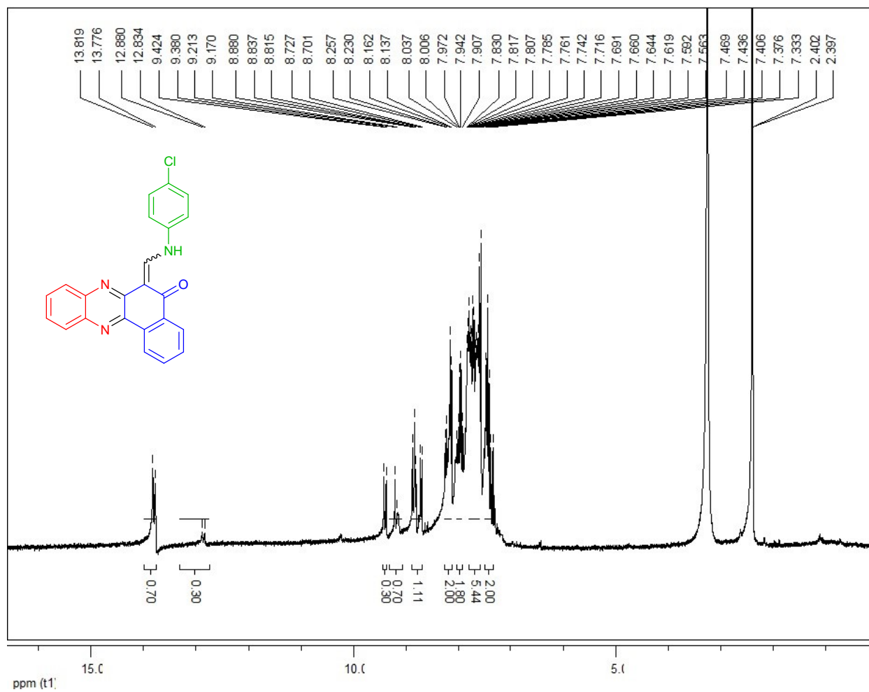
1 H-NMR spectrum of compound 6g (300 MHz, DMSO-d 6 )
