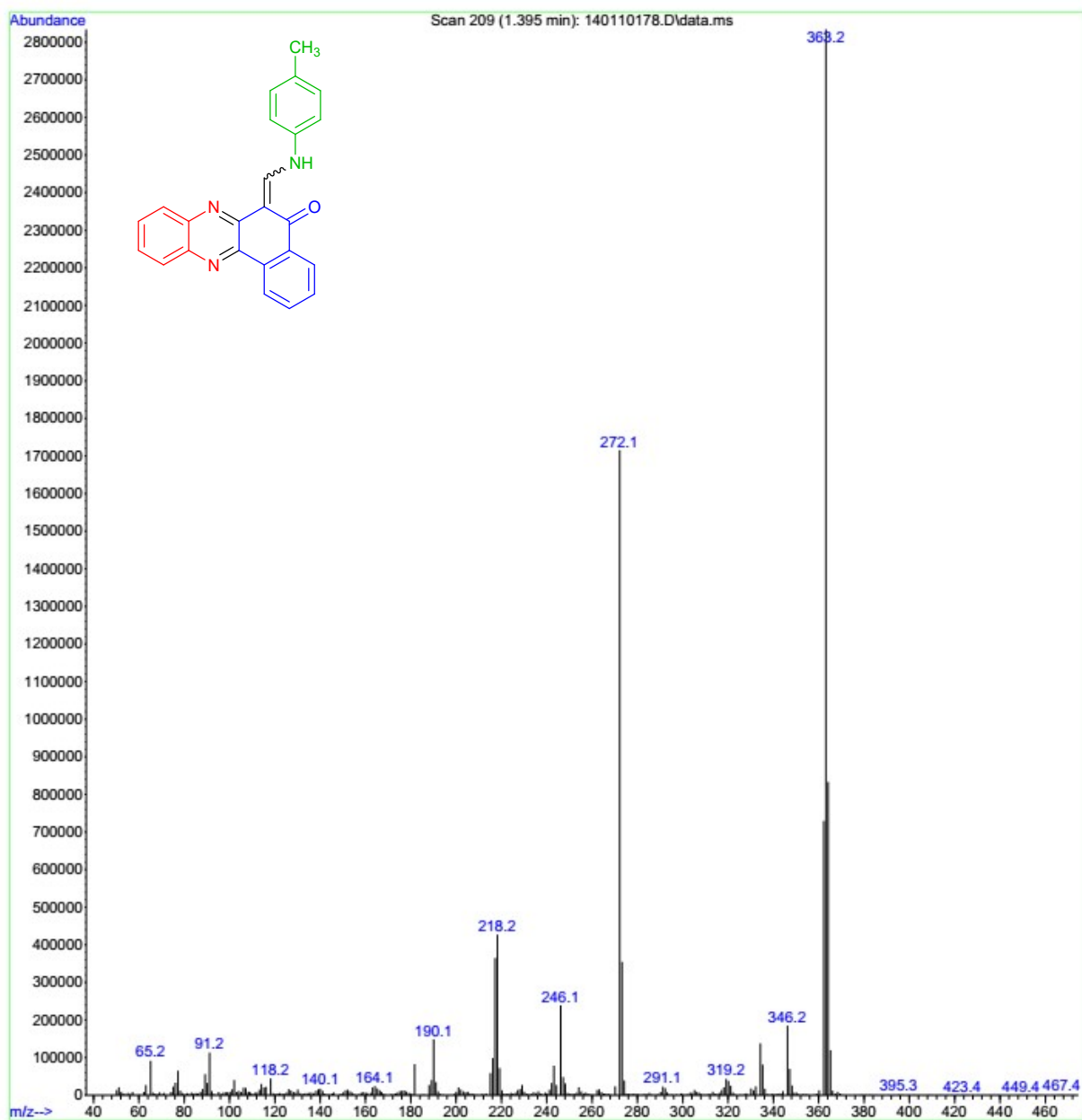
Mass spectrum of compound 6h
