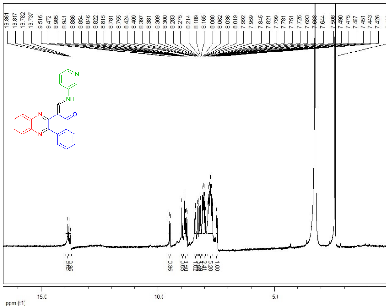
1 H-NMR spectrum of compound 6d (300 MHz, DMSO- d 6 )
