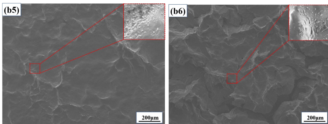
Fig. S2 SEM images of PEG2000 irradiated with (a) 351 and (b) 313 nm UV light for different times: (1) 0 h, (2) 120 h, (3) 240 h, (4) 360 h, (5) 480 h, and (6) 600 h.
