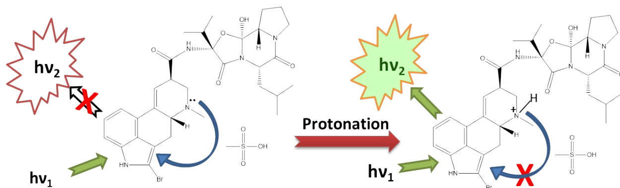
Suppl. (S1) : The mechanism of photo induced electron transfer (PET) and its blocking by protonation
