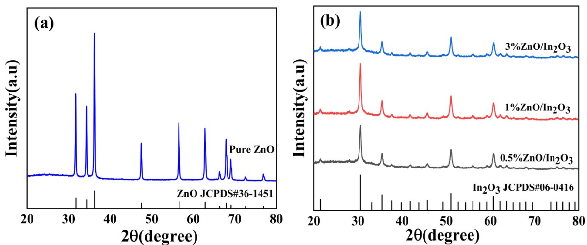
Fig.S2. X-ray diffraction pattern of Pure ZnO, x %ZnO/In 2 O 3 (x=0.5, 1, 3) samples.
