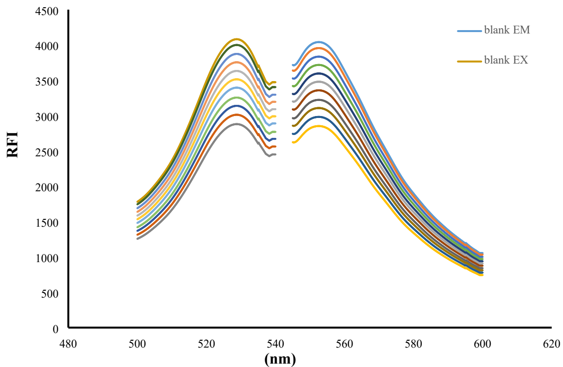
S1 (Figure) Excitation and emission spectra of erythrosine-B ( 2.27 \times 10^{-4} M) and its binary complex with different concentrations of FLX.
