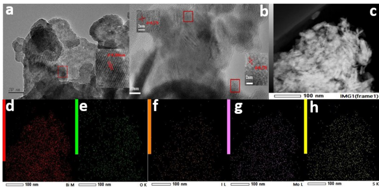
Figure S1. HRTEM images of 3D-FM/BiOI and energy-dispersive X-ray spectroscopy(EDS)(d~h).
