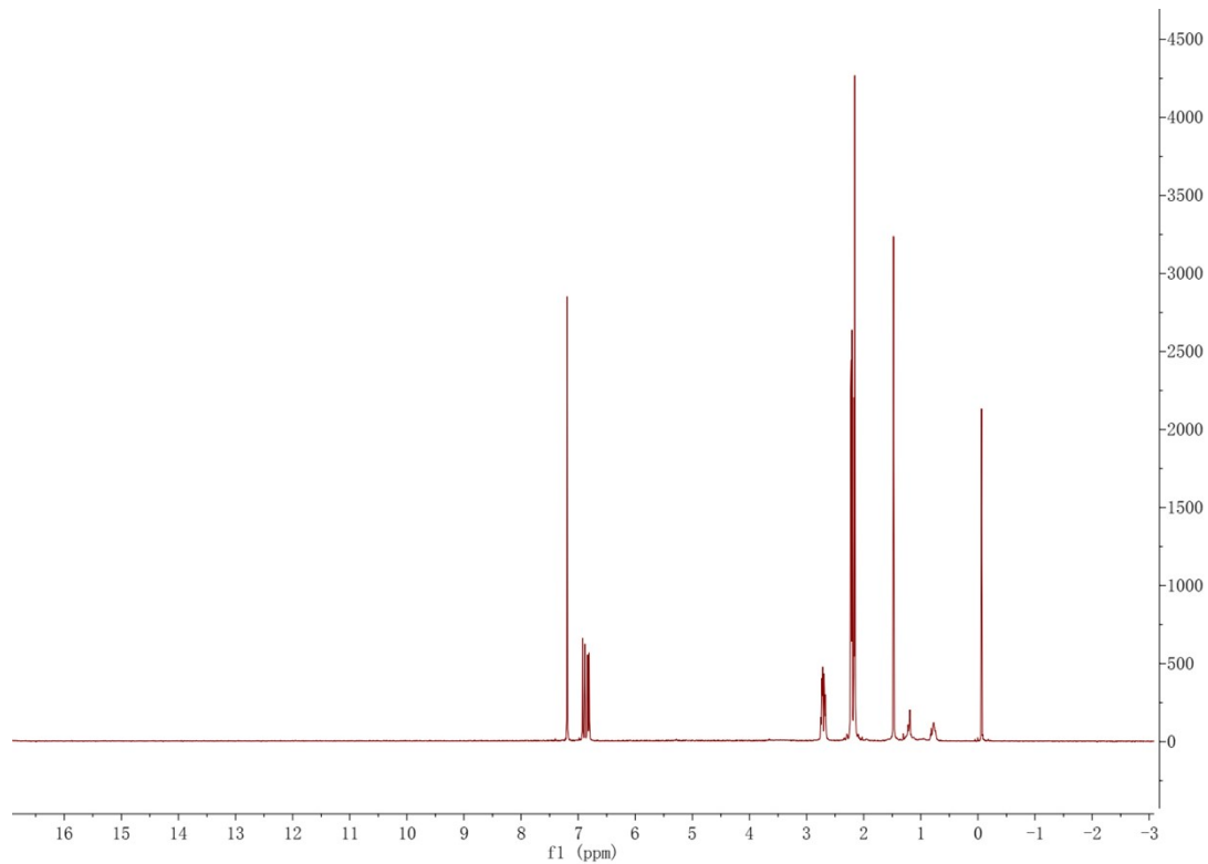
1 H NMR of intermediate 1
