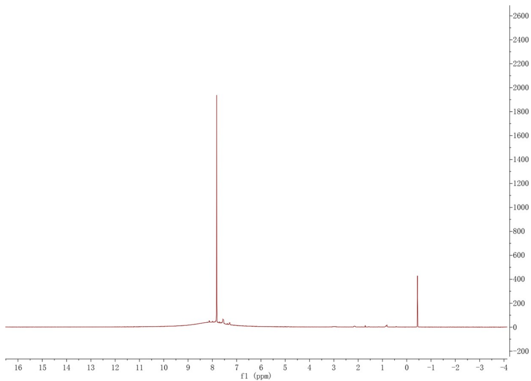
1 H NMR of PMDA
