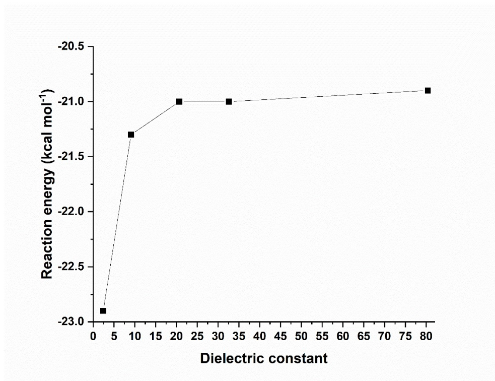
Figure S3. Electronic reaction energy for the association of I-1 with X-TBS for five different solvents (toluene, acetone, water, dichloromethane, methanol) at the \omega B97M-V/def2-TZVP level of theory. All energies are in kcal mol -1 . Free solvation enthalpies were calculated using the C-PCM model.
