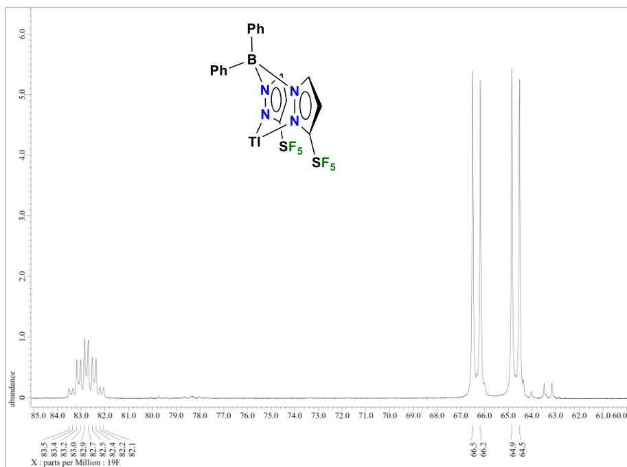
Figure S14: 19 F NMR Spectrum of [\text{Ph}_2\text{B}(3\text{-(SF}_5\text{)Pz})_2]\text{Tl} in \text{CDCl}_3 .
