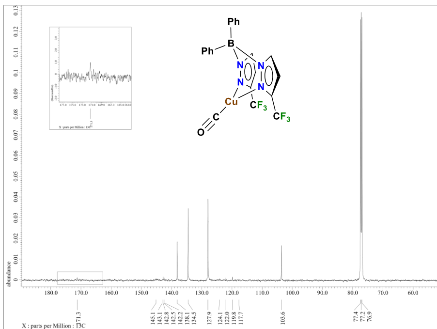
Figure S34: ^{13}\text{C} NMR Spectrum of [\text{Ph}_2\text{B}(3\text{-CF}_3)\text{Pz}]_2\text{Cu}(\text{CO}) in \text{CDCl}_3 .
