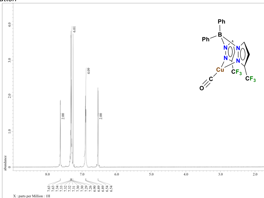
Figure S33: ^1\text{H} NMR Spectrum of [\text{Ph}_2\text{B}(3\text{-CF}_3)\text{Pz}]_2\text{Cu}(\text{CO}) in \text{CDCl}_3
