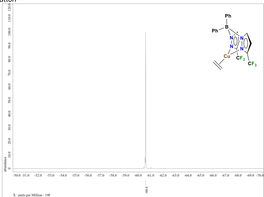
Figure S31: ^{19}\text{F} NMR Spectrum of [\text{Ph}_2\text{B}(\text{3-CF}_3)\text{Pz}]_2\text{Cu}(\text{C}_2\text{H}_4) in \text{CDCl}_3 .
