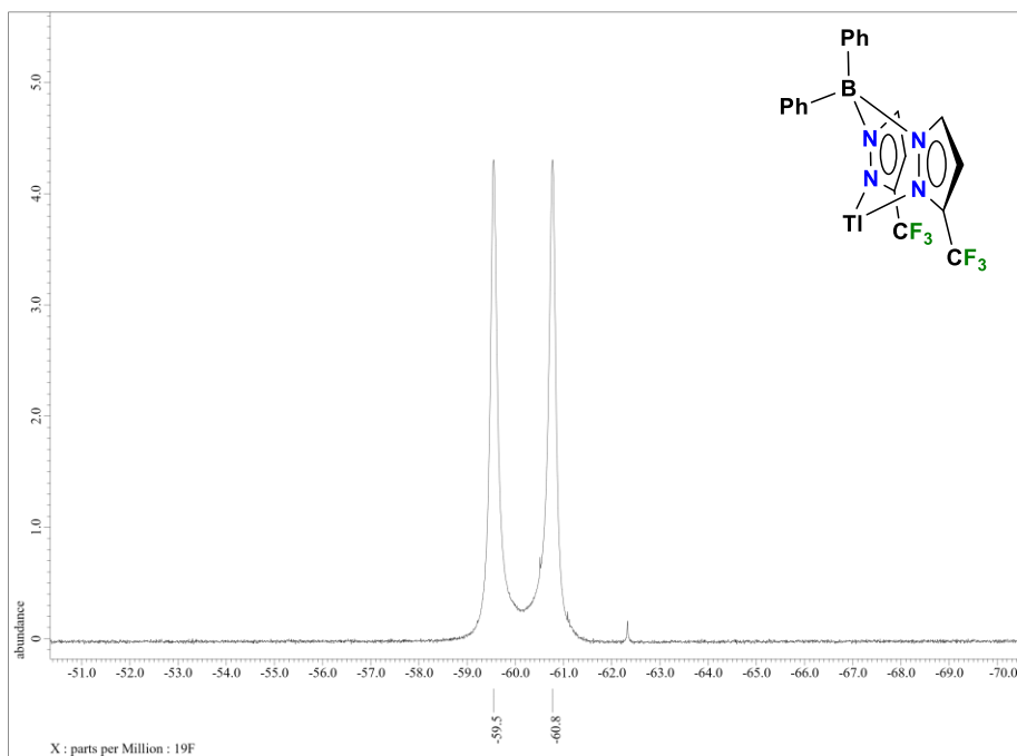
Figure S28: ^{19}\text{F} NMR Spectrum of [\text{Ph}_2\text{B}(\text{3-CF}_3)\text{Pz}]_2\text{TI} in \text{CDCl}_3 .
