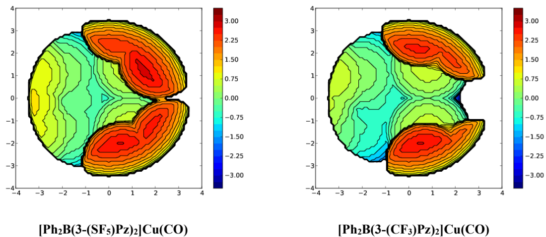
Figure S41: Steric maps of bis(pyrazolyl)borate ligands in [Ph 2 B(3-(SF 5 )Pz) 2 ]Cu(CO) (left) and [Ph 2 B(3-(CF 3 )Pz) 2 ]Cu(CO) (right) based on X-ray data. The resulting % buried volume (%V bur ) values are 68.7 (average of 69.0 and 68.4 for the two molecules in the asymmetric unit) and 60.8 (fluorine atoms of one of the CF 3 groups of [Ph 2 B(3-(CF 3 )Pz) 2 ]Cu(CO) show positional disorder, and only the major occupancy fluorine atoms were utilized in the calculation to avoid inflated steric bulk), respectively. For comparison, inclusion of both disorder-parts in [Ph 2 B(3-(CF 3 )Pz) 2 ]Cu(CO) leads to a marginally higher %V bur value of 61.9.
