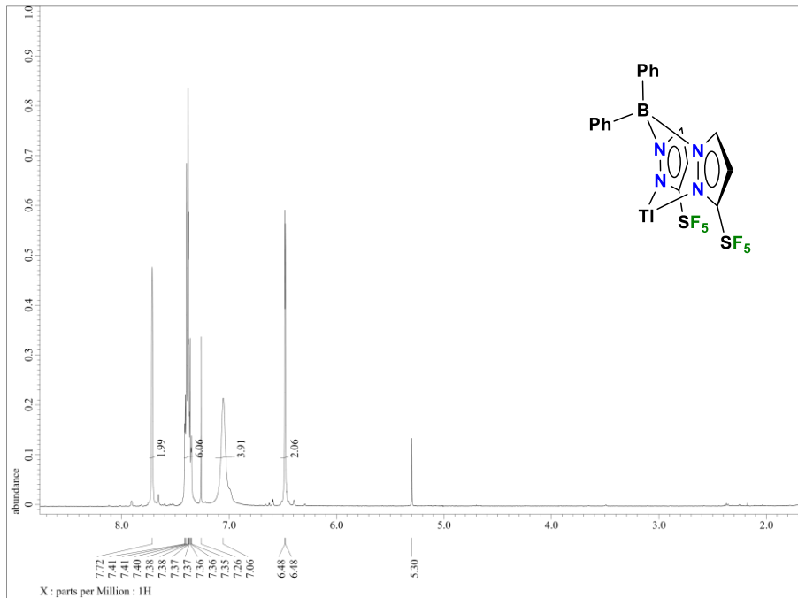
Figure S12: ^1\text{H} NMR Spectrum of [\text{Ph}_2\text{B}(\text{3-(SF}_5\text{)Pz})_2]\text{TI} in \text{CDCl}_3 .
