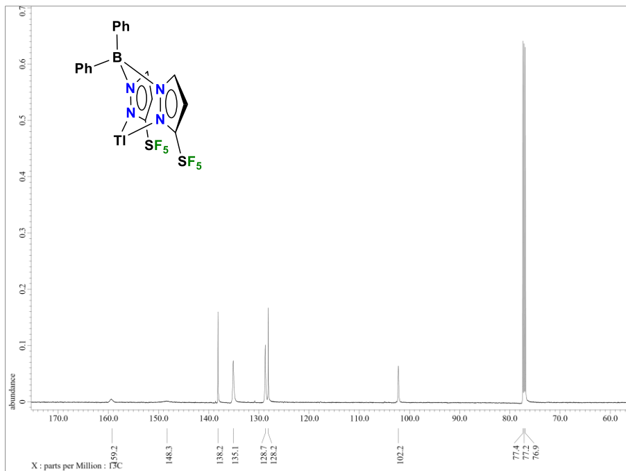
Figure S13: 13 C NMR Spectrum of \text{Ph}_2\text{B}(3\text{-(SF}_5\text{)Pz})_2[\text{Tl}] in \text{CDCl}_3 .
