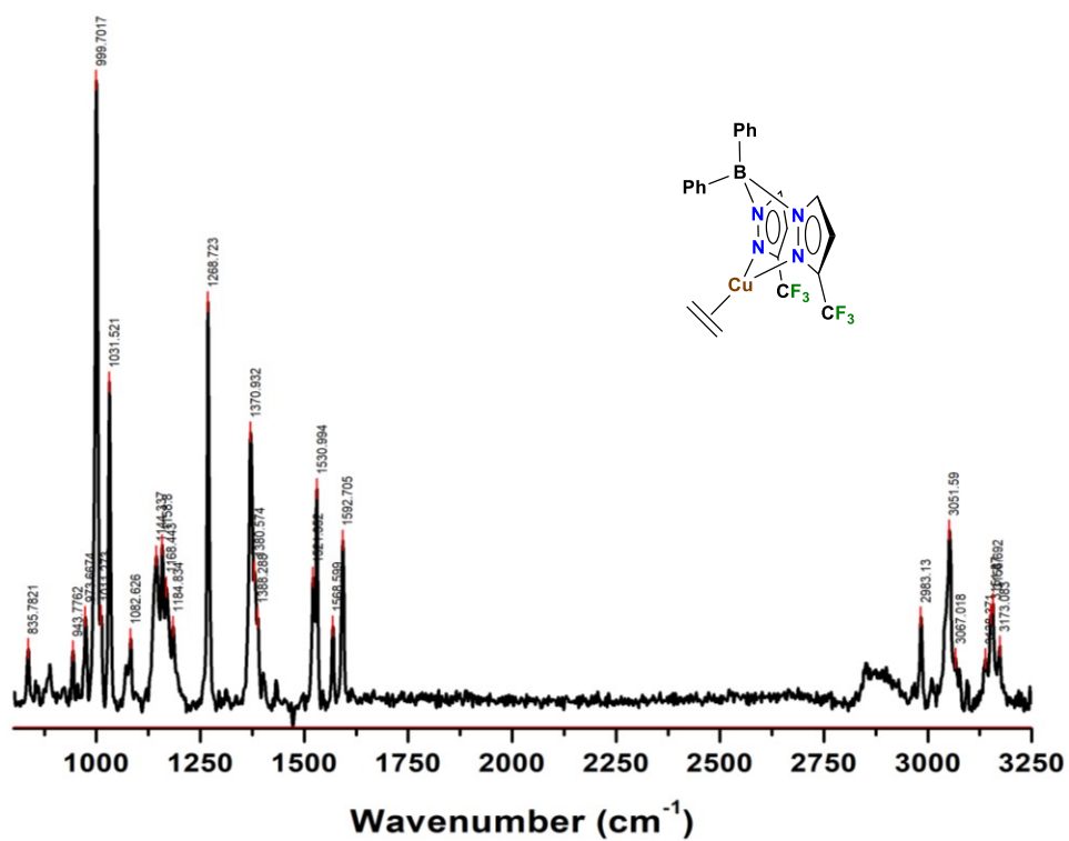
Figure S31: ^{19}\text{F} NMR Spectrum of [\text{Ph}_2\text{B}(\text{3-CF}_3)\text{Pz}]_2\text{Cu}(\text{C}_2\text{H}_4) in \text{CDCl}_3 .
