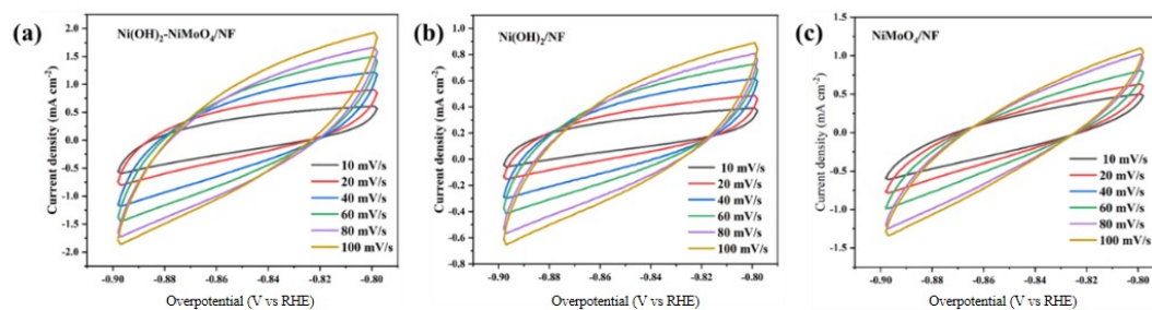
Figure S1. CV plots of Ni(OH) 2 -NiMoO 4 /NF, Ni(OH) 2 /NF and NiMoO 4 /NF in the Faradaic region at different scan rates in 1 M KOH.
