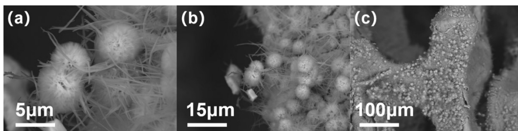
Figure S2. SEM images of Ni(OH) 2 -NiMoO 4 /NF after stability test.
