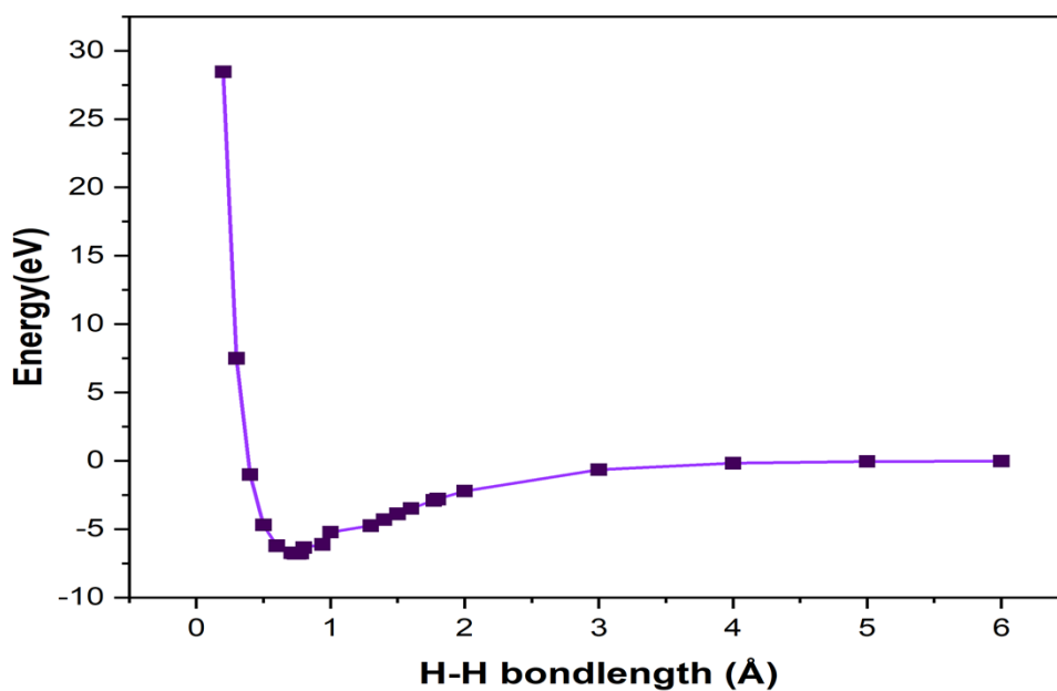
Figure S1: The dissociation curve for isolated H 2 molecule. The optimum bond-length came to be 0.75 Å with an energy of -6.67eV.
