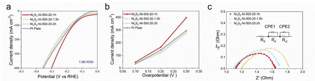
Figure S4. (a) HER polarization curves of Ni 3 S 2 -Ni-500-20-1 h, Ni 3 S 2 -Ni-500-20-1.5 h, Ni 3 S 2 -Ni-500-20-2 h, and Pt plate electrodes. (b) Comparison of the current density of Ni 3 S 2 -Ni-500-20-1h, Ni 3 S 2 -Ni-500-20-1.5 h, Ni 3 S 2 -Ni-500-20-2h, and Pt plate electrodes under the same overpotential. (c) EIS of Ni 3 S 2 -Ni-500-20-1 h, Ni 3 S 2 -Ni-500-20-1.5 h and Ni 3 S 2 -Ni-500-20-2 h electrodes.
